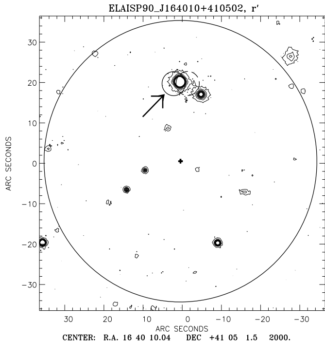
Figure 1. Optical ( r' ) contour map of ELAIS J1640+41 centered on the PHOT detection ( cross ). The lowest contour is drawn at 3\sigma , and then by steps of 6\sigma . The error circle for PHOT ( 35'' ), as well as the 6'' error circles for the detections at 6.7 \mu\text{m} ( solid ) and 15 \mu\text{m} ( dashed ) are also overlaid. The new HyLIG is indicated by an arrow.
