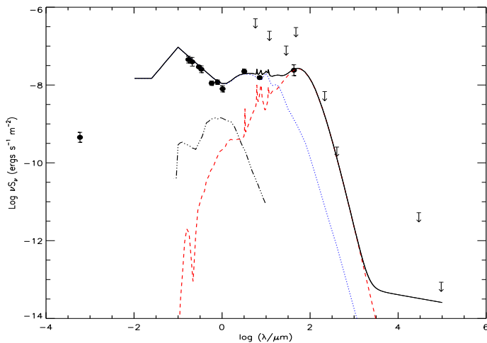
Figure 3. Rest-frame SED of ELAIS J1640+41 from X-rays to radio (data from Table 2). The SED is fitted with a combination of one of the starburst models of Efstathiou et al. (2000b) ( dashed line ; \tau_V = 50 , t = 26 Myrs) and an AGN dusty torus model ( dotted line ) from Efstathiou & Rowan-Robinson (1995). We assume a half-opening angle for the torus of 45^\circ and a face-on inclination. The starburst SED is extrapolated in the radio using the far-IR/radio correlation (Helou, Soifer, & Rowan-Robinson 1985). For the host galaxy, the SED of a 4 Gyr old stellar population ( dotted-dashed line ; Fioc & Rocca-Volmerange 1997) has been normalized to K = 17.0 \pm 0.4 mag (see text).
