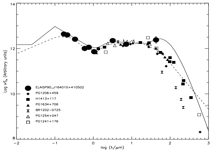
Figure 4. Comparison of the rest-frame SEDs of a number of HyLIGs with optical evidence for quasar activity (data from RR and references therein). The solid and dashed lines show the model fitted to ELAIS J1640+41 (see Fig.3) and the mean SED of radio-quiet quasars in the UVSX sample (Elvis et al. 1994), respectively. The data points are normalized to their rest-frame flux at 15 \mu\text{m} . The vertical scale is arbitrary.
