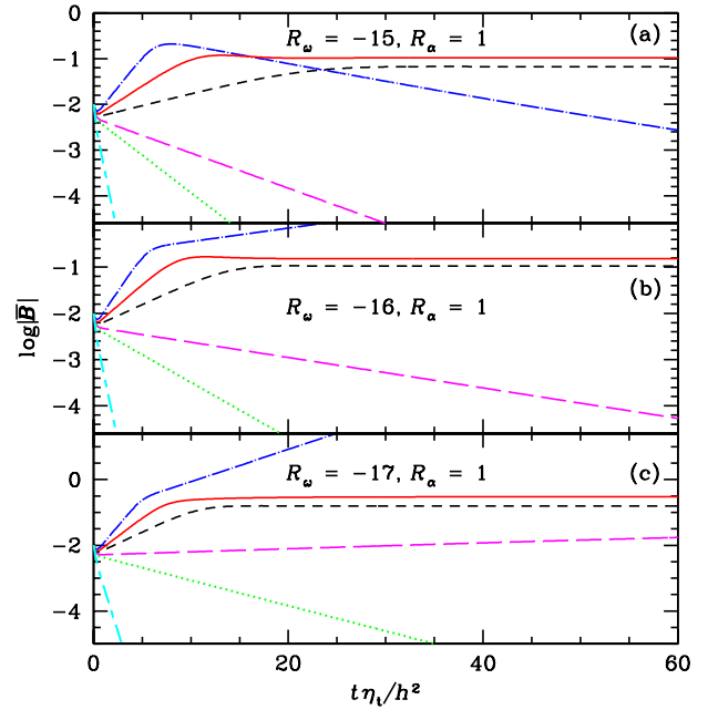
Figure 3. Evolution of the magnetic field strength with both the advective helicity flux and that of Vishniac & Cho, for various magnitudes of the velocity shear: (a) R_\omega = -15 , (b) R_\omega = -16 and (c) R_\omega = -17 . The values of R_U presented are: 0 (dash-dotted), 0.3 (solid), 0.5 (dashed), 0.8 (long-dashed), 1.0 (dotted) and 3.0 (short-long-dashed). The Vishniac-Cho helicity flux supports the dynamo action for larger values of R_U : note decay at R_U = 0.8 in (a) but not in (c). The dynamo action is similarly facilitated for small R_U , where solution with R_U = 0 decays in (a) but not in (b) and (c). The parameters used here are C = 50 , R_m = 10^5 , \overline{B}_\phi|_{t=0} = 10^{-2} and \overline{B}_r|_{t=0} = 0 , with the values of R_\alpha and R_\omega indicated in the legends.
