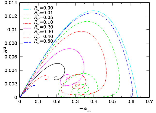
Figure 1. The phase portrait of the dynamical system (14)–(17) in the (\overline{B}^2, -\alpha_m) -plane with and without vertical advection, 0 \leq R_U \leq 0.5 . Parameter values used here are R_\alpha = 1 , R_\omega = -15 , C = 50 , R_m = 10^5 , the values of R_U are shown in the legend, and the time span is t \leq 100h^2/\eta_t .
