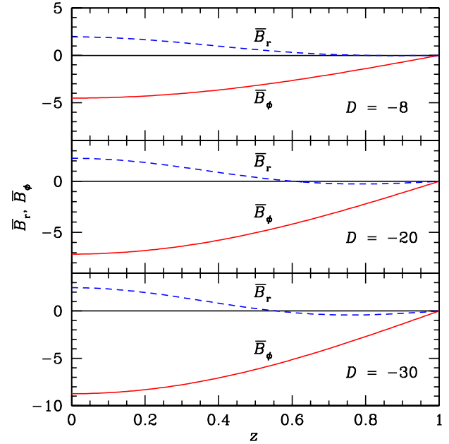
Figure A1. The approximate eigenfunctions \bar{B}_r (dashed) and \bar{B}_\phi (solid) from Eqs (A8) and (A9) for D = -8, -20, -30 (with D_c \approx -8 ), C_0 = 1 and R_\alpha = 1 .
