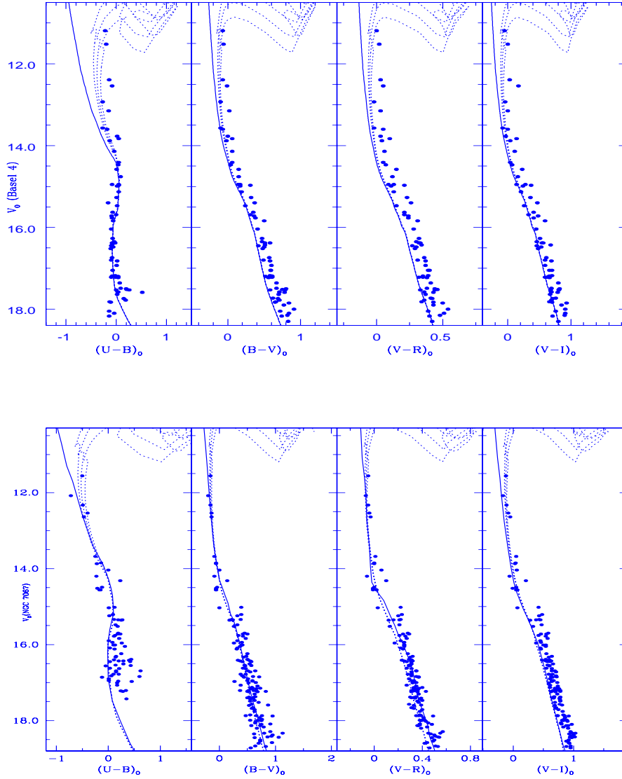
Figure 9. The V_0 , (U - B)_0 ; V_0 , (B - V)_0 ; V_0 , (V - R)_0 and V_0 , (V - I)_0 diagrams for stars of the Basel 4 and NGC 7067. The continuous curves, ZAMS fitted to the MS and dotted curves are the isochrones for Z = 0.008 stars of \log(\text{age})=8.2, 8.3 and 8.4 for Basel 4 and Z = 0.02 stars of \log(\text{age})=7.9, 8.0 and 8.1 for NGC 7067.
