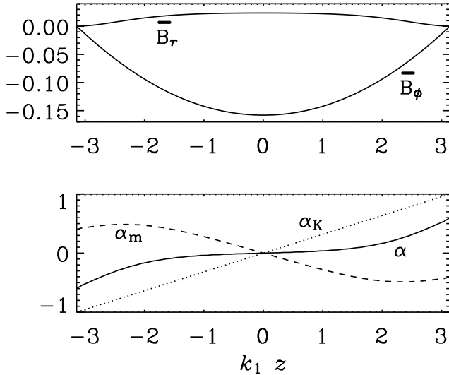
Fig. 2. Plots of \bar{B}_\phi and \bar{B}_r (upper panel) and \alpha (solid), \alpha_m (dashed) and \alpha_K (dotted) (lower panel) versus z in the steady state for C_U = 0.3 , C_\Omega = -2 , C_\alpha = 1 , R_m = 10^5 , and k_1 = \pi/h .
