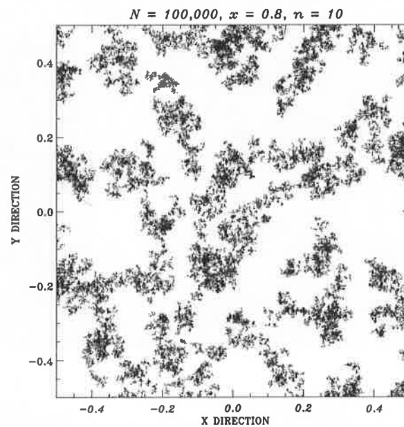
Fig. 2.— A cluster-void distribution generated in the 2D toy model for N = 100,000 initially randomly distributed particles, with typical separation parameter x = 0.8 , and the number of iterations n = 10 . Each particle resembles a galaxy. For further discussion see the text.
