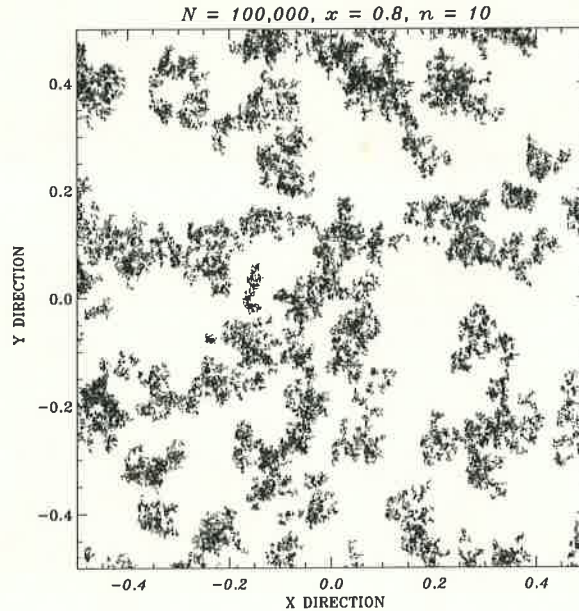
Fig. 4.— A computer simulated filament-void distribution with n(> 2) iterations of aligned ejections having new points following the rule of Figure 3, for the same parameters of Figure 2.
