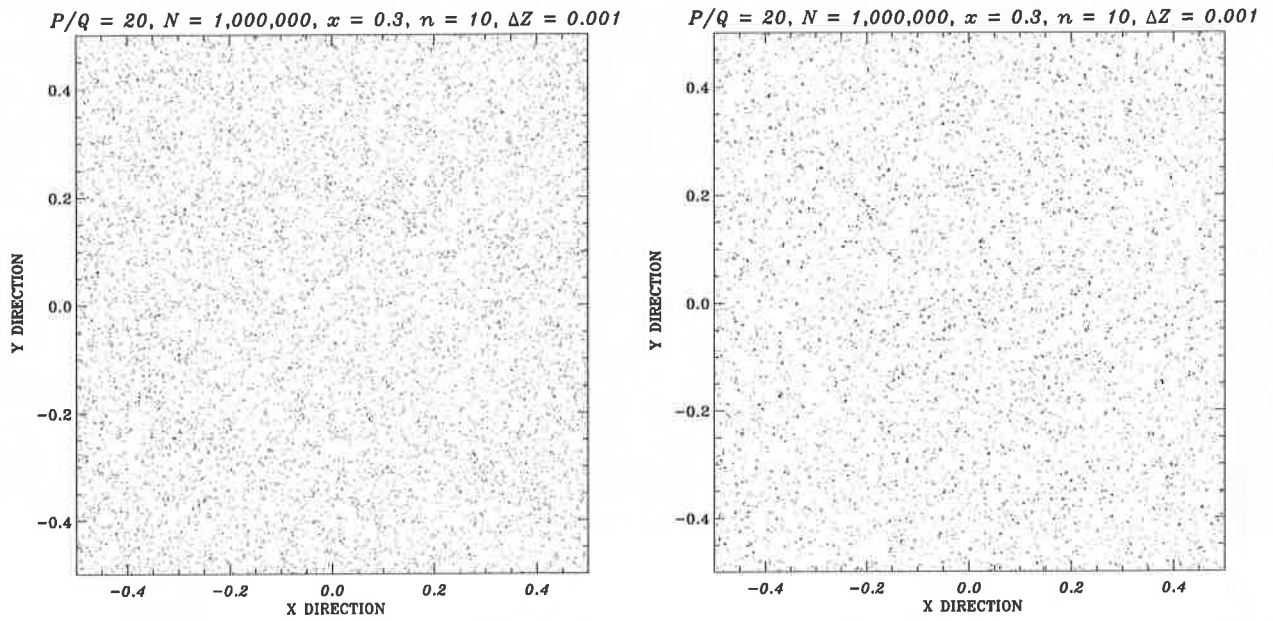
Fig. 6.— A 3-dimensional version, adapted for the QSSC with N = 1,000,000 , x = 0.3 , n = 10 , and P/Q = 20 . Slice thickness in the Z direction is \Delta Z = 0.001 . Evidently, voids are seen separated by filamentary structures. The left panel is for the case of isotropic distribution of particles, whereas the right panel shows the case of aligned ejections.
