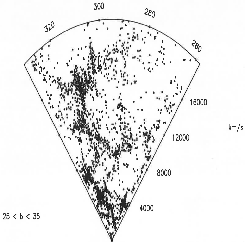
Fig. 7.— A FLAIR redshift survey in the direction of Hydra-Centaurus. Data have been taken from the paper by Raychaudhury, Somak, Colless, M., & Holo, R., 1994, proceedings of the 35th Herstmonceux Conference on Wide-Field Spectroscopy and the Distant Universe , Cambridge 1994, World Scientific.
