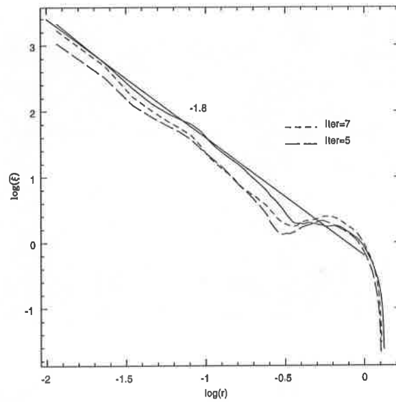
Fig. 8.— The two point correlation function for the QSSC based model. Here, N = 100,000 and x = 0.3 . As “time” goes on, the curve approaches more and more closely the slope of -1.8 . The solid curve shows the result after 10 iterations.
