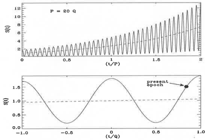
Fig. 1.— The scale factor S(t) of the QSSC in the upper panel against t to show how several oscillatory cycles of short period Q are accommodated in the longer e -folding time P of the exponential expansion. In the lower panel are sketched a few oscillations on an expanded timescale with our present epoch marked. The parameter values have been taken from those given in section 2.3.
