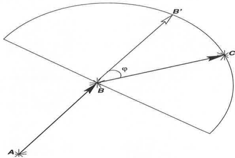
Fig. 3.— Here we schematically show the procedure for creating units in aligned direction for n > 2 . Particle A is a representative of first generation units which are distributed randomly. B is a representative of the second generation units, being created in a random direction. Point C represents a third generation unit which has been created in the half plane lying away from A off the line perpendicular to AB . BC therefore makes an acute angle, \varphi , with the line ABB' .
