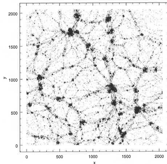
Fig. 5.— A power law 2D simulation in the standard big bang cosmology for power index, n = -0.4 of density fluctuations.
