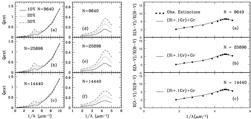
Figure 1. Extinction efficiency of the Composite Grains (left panel) and comparison with observed interstellar extinction curve (right panel).
