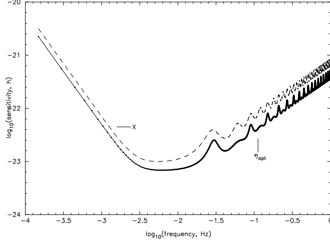
FIG. 6: The LISA Michelson sensitivity curve (SNR = 5) and the sensitivity curve for the optimal combination of the data, both as a function of Fourier frequency. The integration time is equal to one year, and LISA is assumed to have a nominal armlength L = 16.67\text{sec} .
