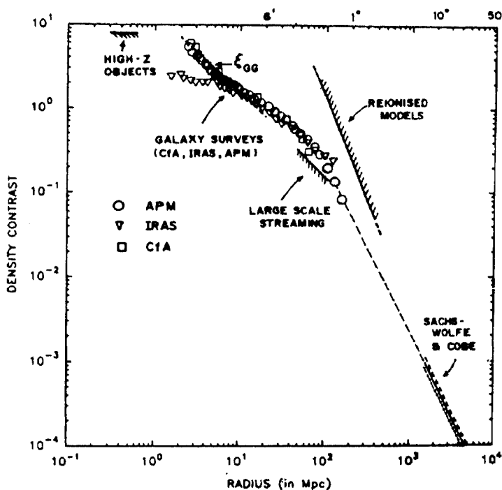
Figure 4. Various constraints on the rms fluctuations in mass, \sigma(R) = \langle (\delta M/M)^2 \rangle^{1/2} , are plotted against the scale R . Within a factor or order unity, this \sigma^2(R) also represents the power in each octave, [k^3 P(k)/2\pi^2] , at k = R^{-1} . At the right-bottom, the result from COBE based on (\Delta T/T)_{\text{rms}} is marked assuming a spectrum which is scale-invariant at large scales. The \sigma(R) determined from CfA, IRAS and APM surveys are shown by different symbols. In the case of APM, W(\theta) was inverted to give \zeta(r) . We have not included QDOT data in this figure because it is based on cubical cells. The lower bound on \sigma(R) —marked 'high- z objects'—arises from requiring that mass scales in the range (10^{10}-10^{11}) M_\odot should go nonlinear by z=4.5 . The bound marked 'large scale streaming' arises from the POTENT reconstruction of velocity fields. We have also shown the (rather weak) upperbound from small angle anisotropies in MBR in the reionized models and the slope of the galaxy-galaxy correlation function ( h=0.5 ).
