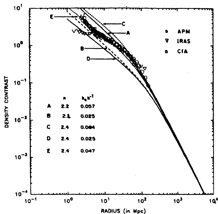
Figure 5. The results of galaxy surveys and COBE anisotropy are fitted using simple test spectra of the form P(k) = Ak [1 + (k/k_c)^n]^{-1} . All the spectra are normalized using the maximum permitted value of a_2 from COBE, viz. a_2 = 10^{-5} . There is reasonable agreement for n=2.4 , k_c=0.047 h (the fit can be marginally improved by choosing n=2.41 and k_c=0.047 h ). This suggests a length scale of k_c^{-1}=21 h^{-1} Mpc in the theory. We have set h=0.5 .
