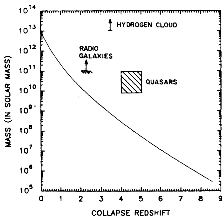
Figure 3. The mass scale which goes nonlinear at various redshifts is shown for a CDM model with \sigma_8 \approx 0.5 , h=0.5 . Also shown are the masses of several high redshift objects.
