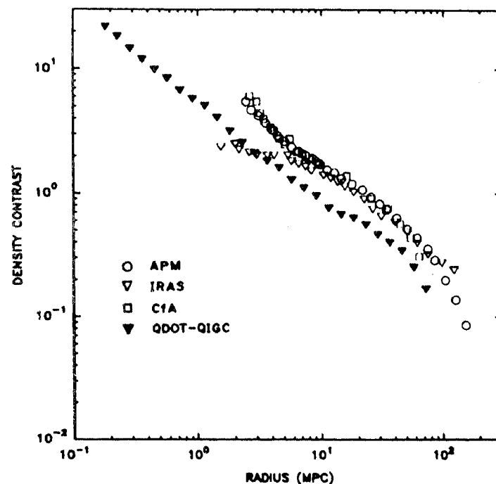
Figure 2. The density contrast \sigma(R) = \langle (\delta M/M)^2 \rangle_R^{1/2} determined from various galaxy surveys (see ref. 20): APM (circles), IRAS (open triangles), CfA (squares) and QDOT (filled triangles). The QDOT results are based on counts in cubical cells of size R while the other three results are based on spheres of radius R , which could partly account for the systematic shift. The QDOT data were kindly provided by Rowan-Robinson and is based on Saunders, W. et al. , 1992 (Oxford preprint OUTAS/92/4; to be published). We have set h = 0.5 .
