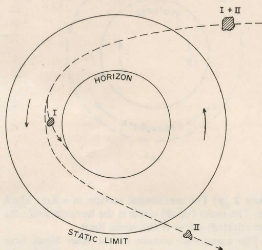
Figure 3 Penrose's scheme of extracting energy from a rotating black hole by diminishing the black hole's angular momentum. The final residual mass (II) which emerges has greater energy than the total mass (I+II) which went into the ergosphere.
