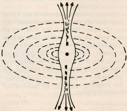
Figure 5 The twin exhaust model of Blandford and Rees. The plasma is squirted out along the two nozzles aligned with the axis of rotation.
