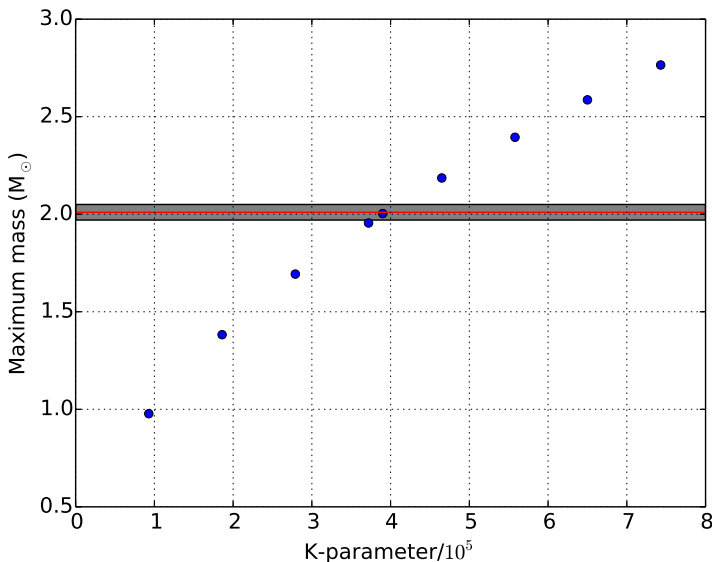
FIG. 1. The maximum gravitational mass of a BEC star obeying the CSW equation of state [15] is plotted as a function of the free parameter K (in \text{cm}^5 \text{g}^{-1} \text{s}^{-2} ) in (blue) dots. The thin horizontal (red) line shows the observed maximum mass of a neutron star and the horizontal gray band shows the error in that value [6]. Since the dots intersect the line at K = 3.7169 \times 10^5 \text{ cm}^5 \text{g}^{-1} \text{s}^{-2} , this is the minimum value of K allowed by observations of neutron star masses.
