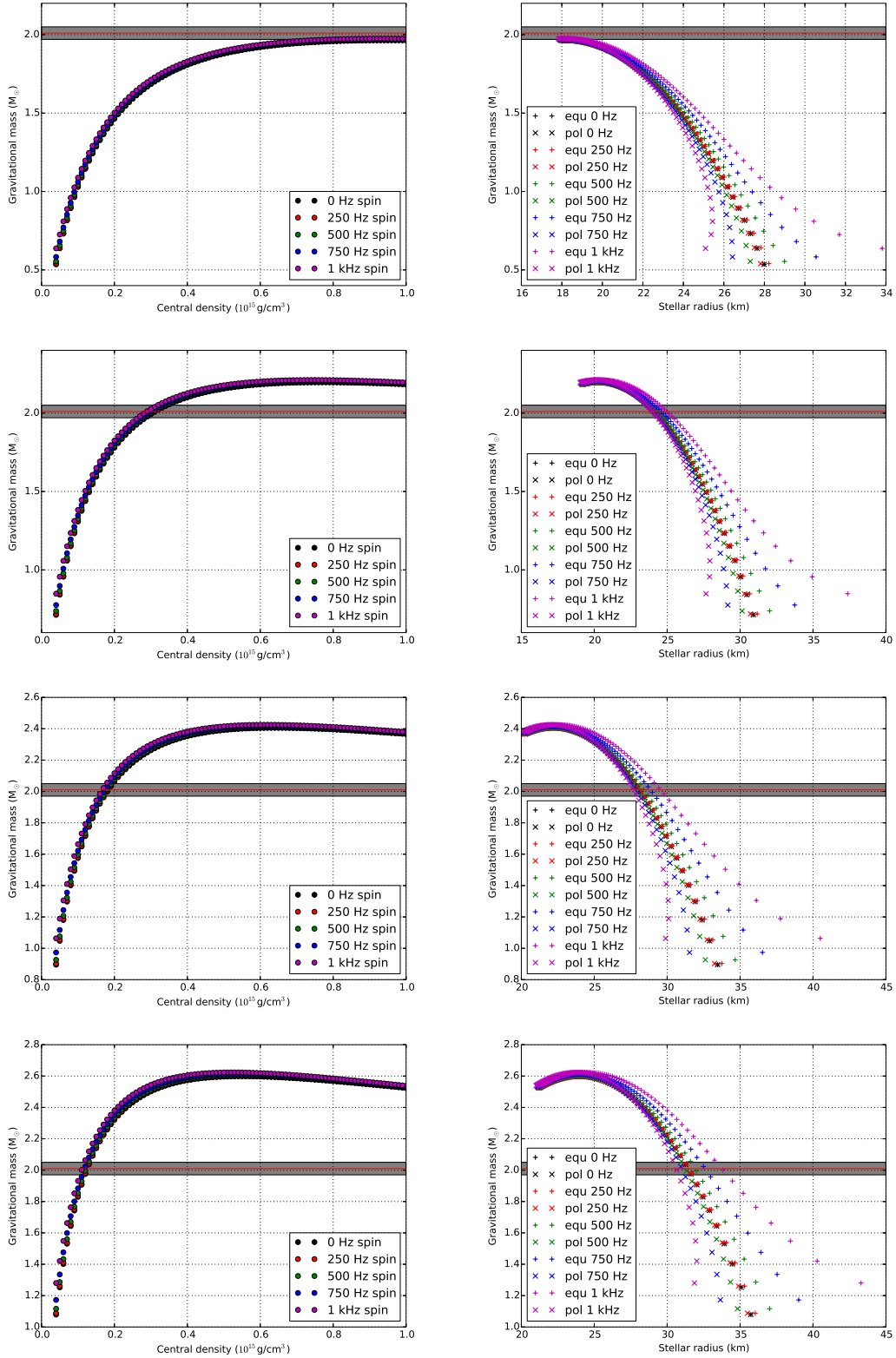
FIG. 3. The gravitational mass of neutron stars with a variety of spin frequencies and obeying the CSW EOS are plotted as a function of the central-density (left-column) and radius (right-column). Each row corresponds to a different value of the CSW EOS parameter (in \text{cm}^5 \text{ g}^{-1} \text{ s}^{-2} ): K = 3.72 \times 10^5 (top row), 4.65 \times 10^5 (second row), 5.58 \times 10^5 (third row), and 6.50 \times 10^5 (bottom row). The equatorial (“equ”) and polar (“pol”) radii for a variety of neutron star spins (including the non-spinning “0 Hz spin” case) are also shown here.
