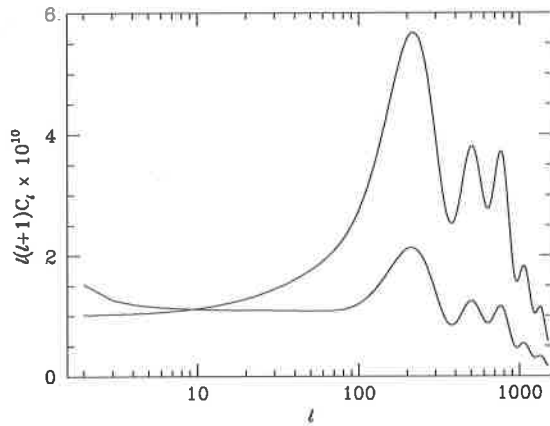
Figure 1. Angular power spectrum for a critical density Universe with cold dark matter, \Omega_b = 0.05 and spectral index n = 1 (upper panel), n = 0.85 (lower panel). (Figure courtesy of M. White.)
