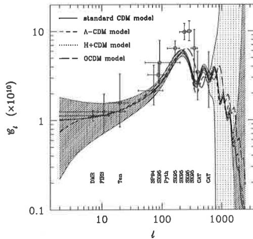
Figure 2. CMB anisotropy expected in several theoretical models CDM, H+CDM, \Lambda -CDM and Open CDM. Also shown are CMB anisotropy measurements from some recent experiments (details are in Page 1997). The tilted solid shading shows the expected performance of MAP and Planck Surveyor satellite missions. (Figure courtesy of T. Souradeep.)
