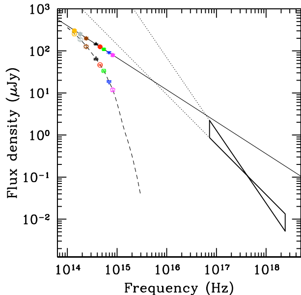
Figure 3. SED of the afterglow of GRB071010A about 0.8 d after the burst. The dashed line is a fit to the observed data in the optical/NIR. The solid line refers to the intrinsic SED once the effect of dust absorption in the Milky Way and in the GRB host galaxy is removed. The X-ray and optical/NIR broad-band SED is consistent with the predictions of the synchrotron external-shock scenario with a cooling break between the optical/NIR and the X-ray and \beta_{\text{X}} = \beta_{\text{opt}} + 1/2 .
