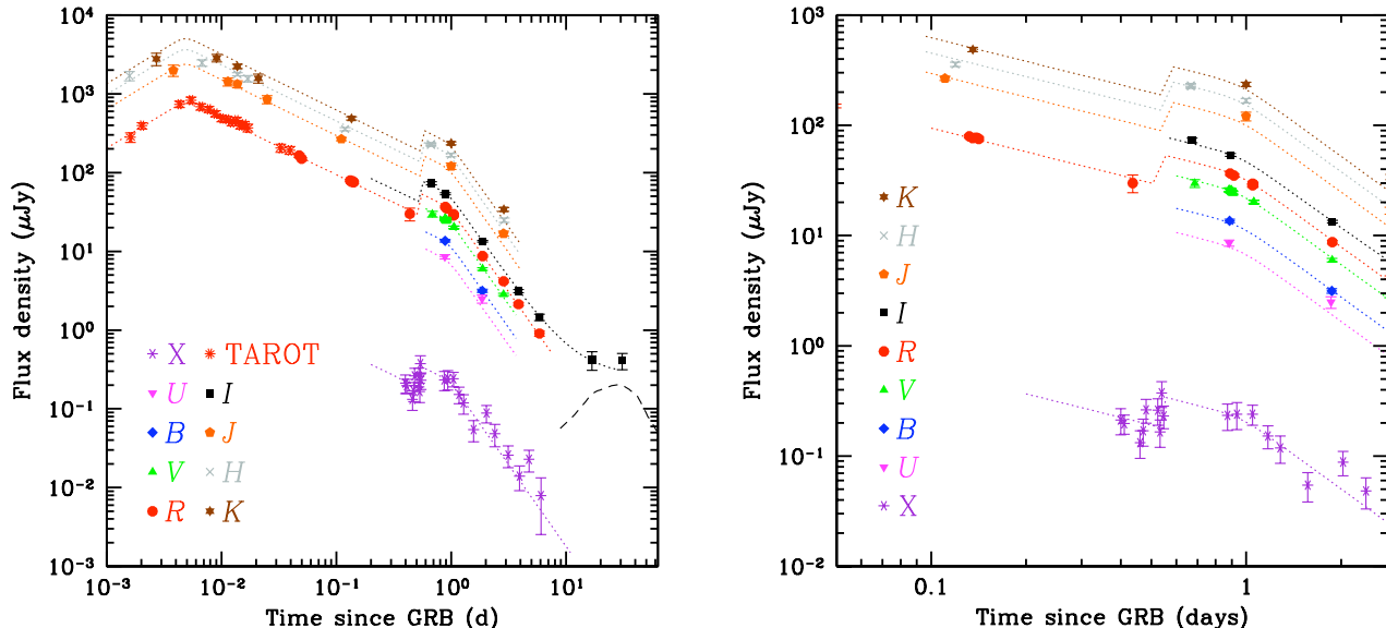
Figure 2. The optical, NIR, and X-ray light curves of the afterglow of GRB071010A. The dashed lines show the fit to the temporal decay of the early and late-time afterglow. Fit parameters are reported in Sect. 3. On the left we show the whole light curve fitted with the adopted model. On the right the epoch around 1 d is magnified. At late times, the long-dashed line shows the possible contribution to the I band by a supernova component using SN 1998bw (Galama et al. 1998) as a template, at the redshift of GRB 071010A. The effect of the absorption in the optical is included.
