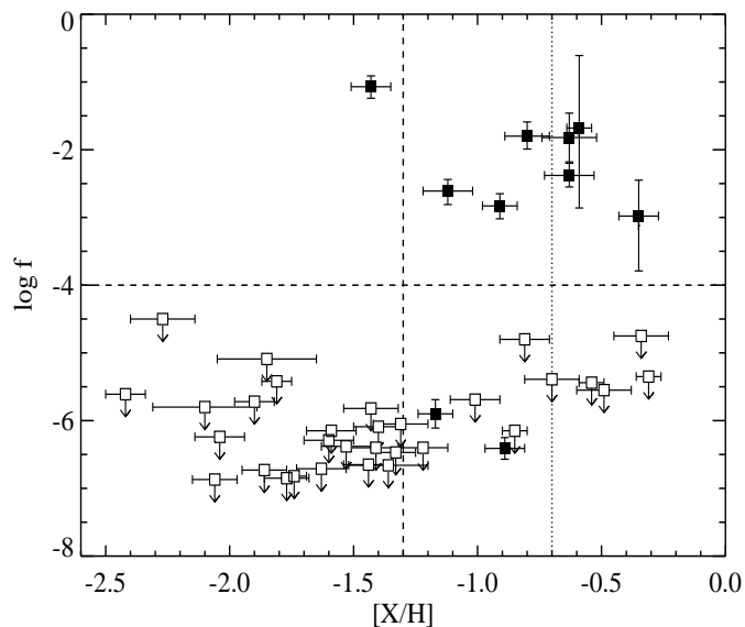
Fig. 3. Logarithm of the molecular fraction, f = 2N(\text{H}_2)/(2N(\text{H}_2) + N(\text{H I})) , versus metallicities, [X/H] = \log N(X)/N(H) - \log(X/H)_\odot and X either Zn, S or Si, in DLAs from the sample described in this paper ( [X/H] > -1.3 , see Table 1) and the sample of Ledoux et al. (2003, [X/H] < -1.3 ). Filled squares indicate systems in which H 2 is detected. Dashed lines indicate the limits used in the text ( \log f = -4 ; [X/H] = -1.3 ). The dotted line indicates the median of the high-metallicity sample ( [X/H] = -0.7 ).
