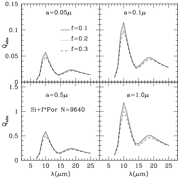
Fig. 9. Variation of Absorption Efficiencies with composite grain sizes. Host silicate spheroids contain dipoles N=9640 and voids (vacuum) as inclusions
