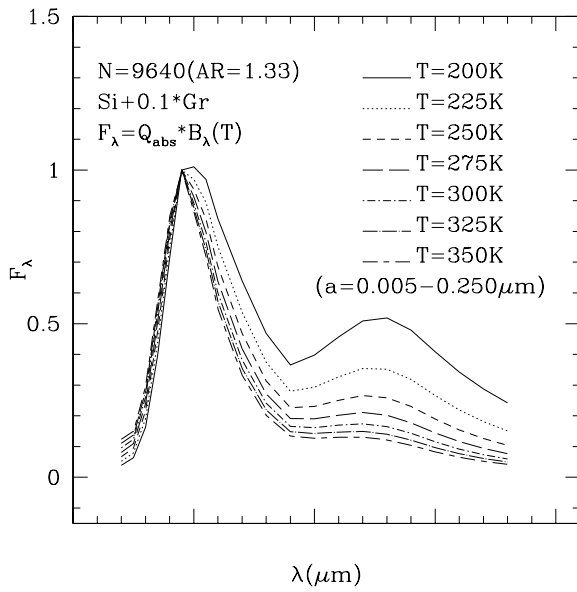
Fig. 10. Infrared Flux at various temperatures, for the composite grains with graphites as inclusions
