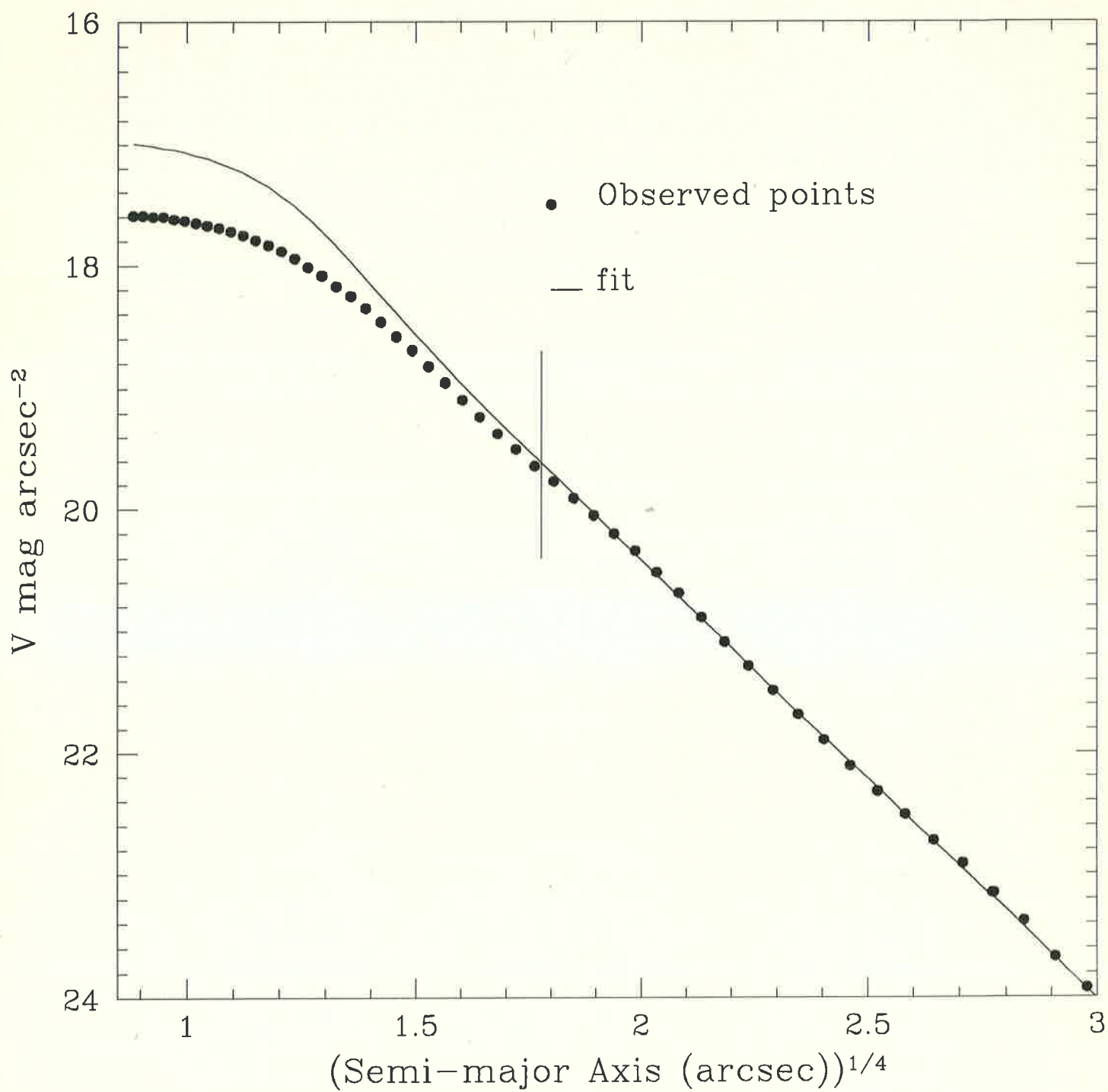
Figure 4 : Observed brightness profile along the semi-major axis, and a de Vaucouleurs' law fit made using points beyond the small vertical bar shown at a = 11'' . The fit is extrapolated to the region inward of the bar. Deviation of the fit from the observed points in the inner region is indicative of the extinction due to dust.
