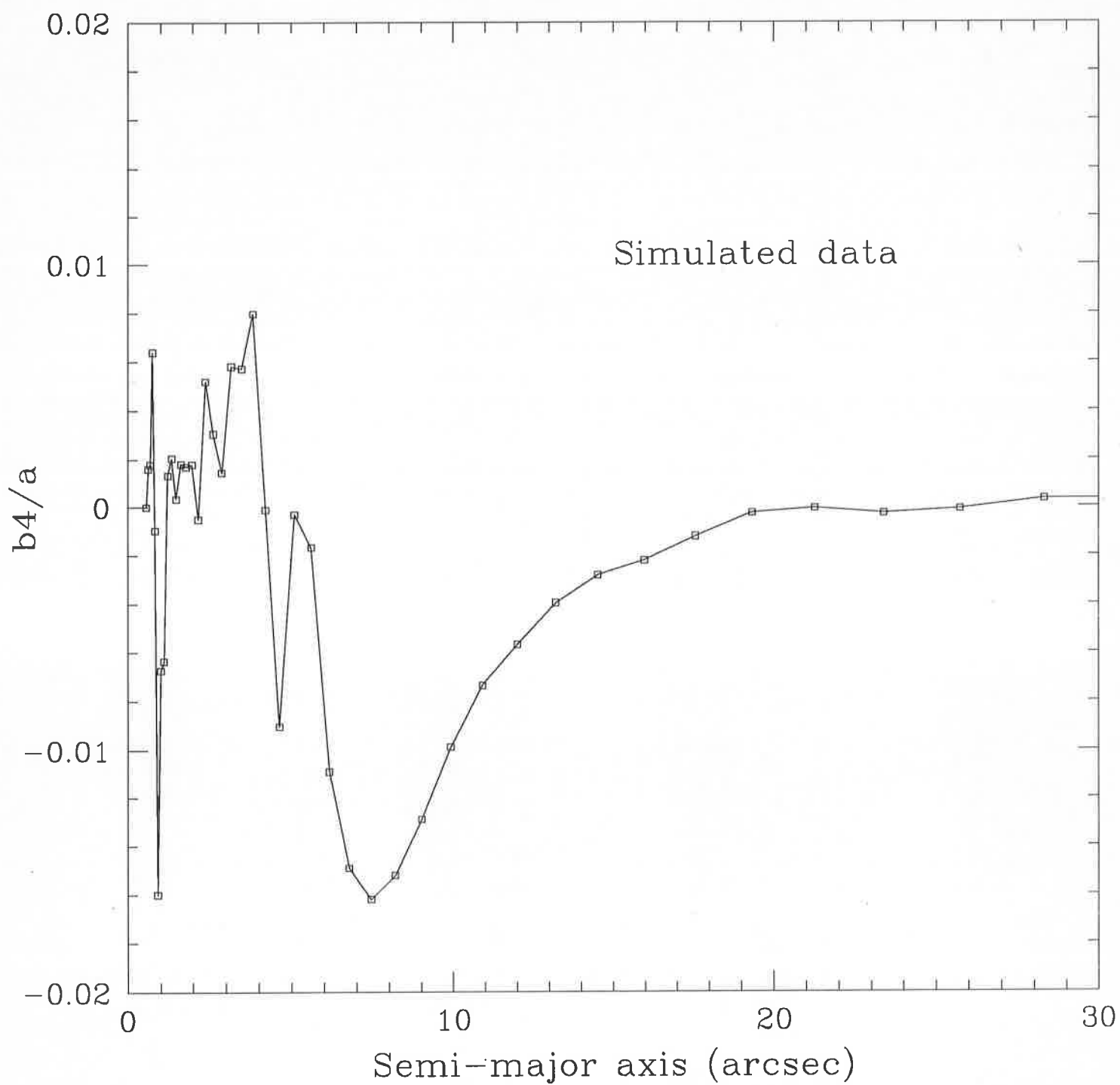
Figure 6 : The boxiness coefficient for a simulated elliptical galaxy generated using the parameters obtained for NGC 4261.
