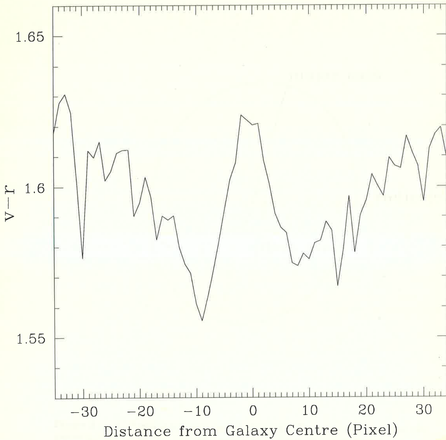
Figure 2 : A cut across the dust lane, averaged over 10 rows around the galaxy centre. The instrumental colour v - r is shown.
