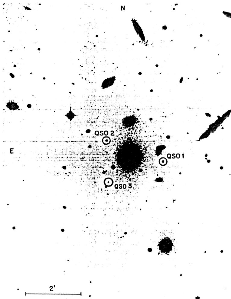
FIGURE 6. THREE MORE HIGH-REDSHIFT QUASARS found within 2 arcminutes of the center of a local, low-redshift galaxy, NGC 3842. Halton Arp was involved in the discoveries of all three. 17 Once again, we argue that such superposition is very unlikely to be accidental.
