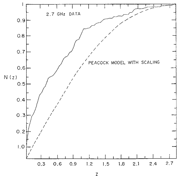
FIG. 10. N(z) curve from Peacock's model (Peacock 1985) against observational N(z) . The absolute numbers produced by the luminosity function of Peacock have been scaled to match the maximum value of N(z) at Z_{\max} = 2.852 , the highest redshift in the 2.7 GHz sample. The dashed line has been obtained from Peacock's model.
