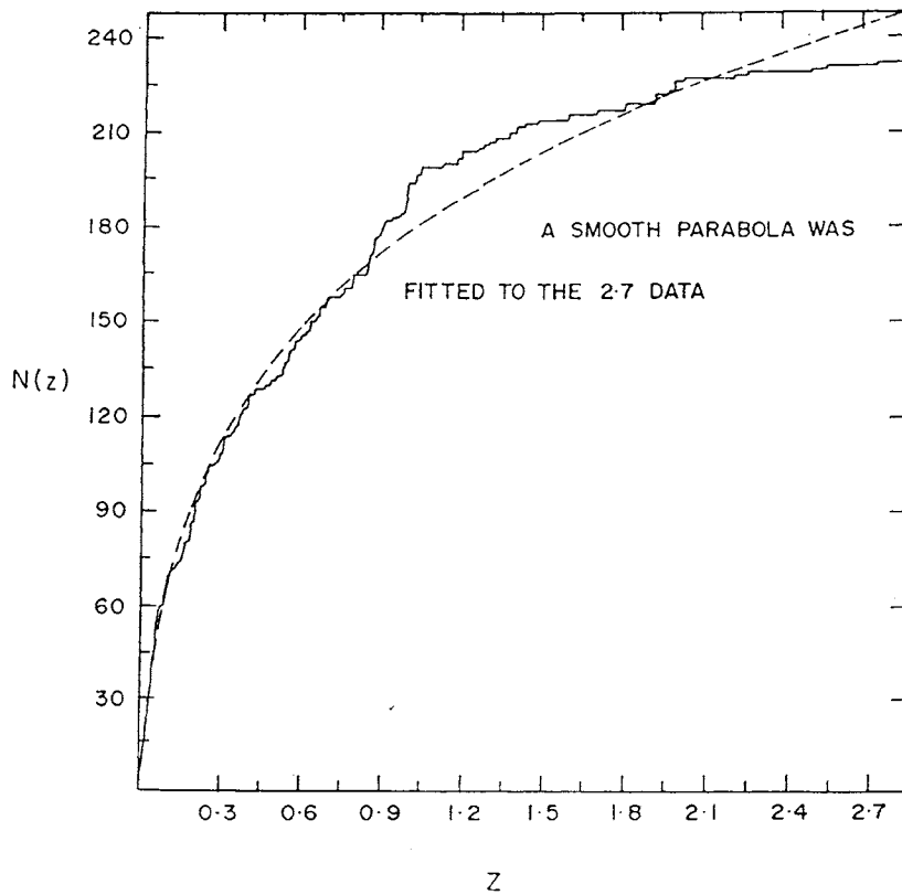
FIG. 7. N(z) - z plot for 2.7 GHz sources (the continuous line is the observational curve, and the dashed line is the least-square fit to the observations).
