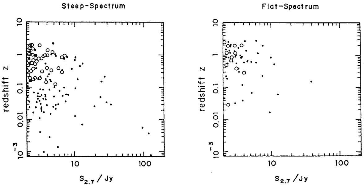
FIG. 2. \log S_{2.7} / \text{Jy} - \log z planes for steep- and flat-spectrum sources. Light circles denote estimated redshifts. Figure based on Wall and Peacock (1985).
