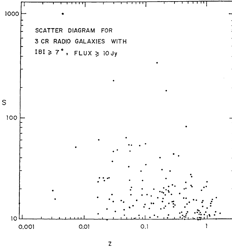
FIG. 1. Scatter diagram obtained by plotting \log z against \log S for the 3CR radio galaxies with |b| \geq 7^\circ and S > 10 Jy.
