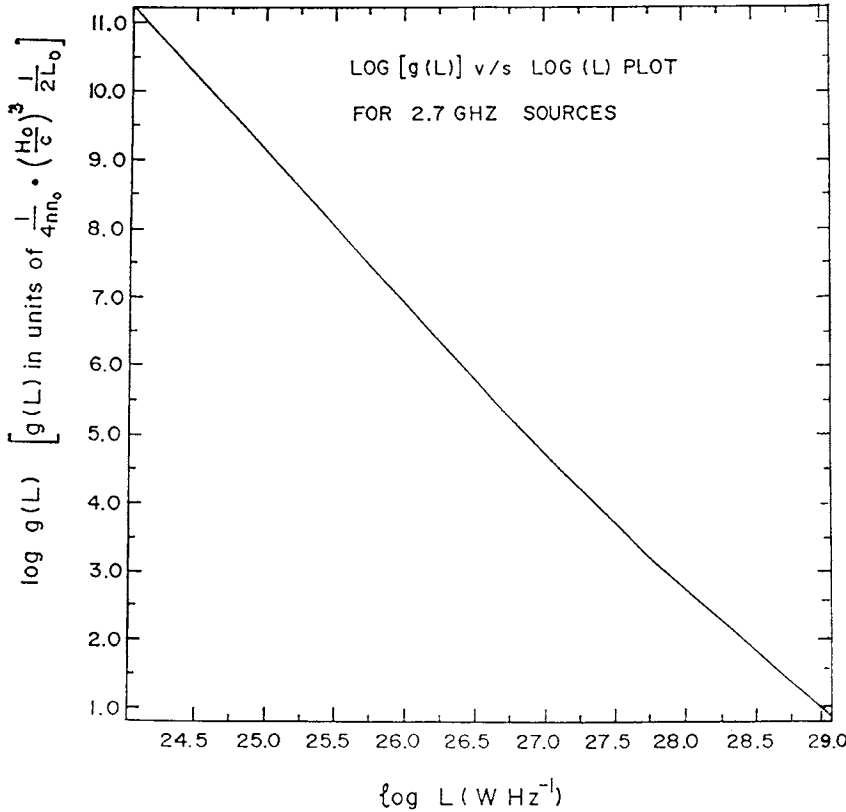
FIG. 8. Plot of \log g(L) against \log L for 2.7 GHz sources.
