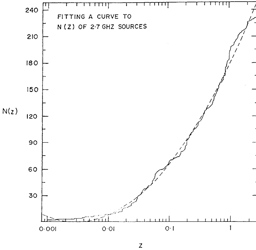
FIG. 6. N(z) - \log z plot for 2.7 GHz sources (the continuous line is the observational curve, and the dashed line is the least-square fit to the observations).
