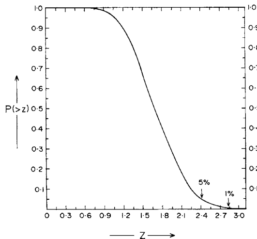
FIG. 9. Empirical cumulative probability distribution of the K-S statistic Z based on one thousand Monte Carlo simulations of the ( z - S ) plot produced by the non-evolving RLF of Fig. 4.
