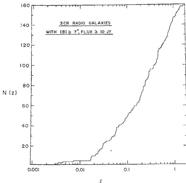
FIG. 3. Plot of N(z) against \log z for 3CR radio galaxies with |b| \geq 7^\circ , flux \geq 10 Jy. At high z , the curve shows indications of flattening.
