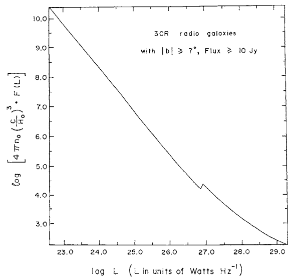
FIG. 4. Plot of \log F(L) against \log L for 3CR radio galaxies with |b| \geq 7^\circ , flux \geq 10 Jy. The discontinuity at \log L \sim 27 is not physically significant and arises from the two-straight-line approximation of Eqs. (19) and (20).
