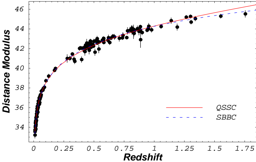
Fig. 2. Best-fitting flat models in QSSC and SBBC are compared with the ‘gold sample’ of SNe Ia data from Riess et al. 20 The QSSC model corresponds to \Omega_{\Lambda 0} = -0.2 .
