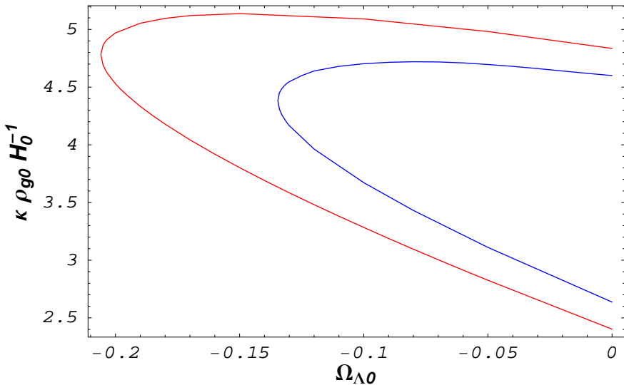
Fig. 1. The allowed regions by the ‘gold sample’ of SNe Ia data (with 157 points) are shown at the 95% (inner contour) and 99% (outer contour) confidence levels, by marginalizing over \mathcal{M} (the parameters \kappa, \rho_{g0} and H_0 are measured in units of 10^5 \text{ cm}^2 \text{ g}^{-1}, 10^{-34} \text{ g cm}^{-3} and 100 \text{ km s}^{-1} \text{ Mpc}^{-1} respectively). For the average values \kappa = 5 \times 10^5 \text{ cm}^2 \text{ g}^{-1} and H_0 = 70 \text{ km s}^{-1} \text{ Mpc}^{-1} , the estimated range of the whisker grain density from the data is 3.5 \times 10^{-34} \text{ g cm}^{-3} \leq \rho_{g0} \leq 8 \times 10^{-34} \text{ g cm}^{-3} at 99% confidence level.
