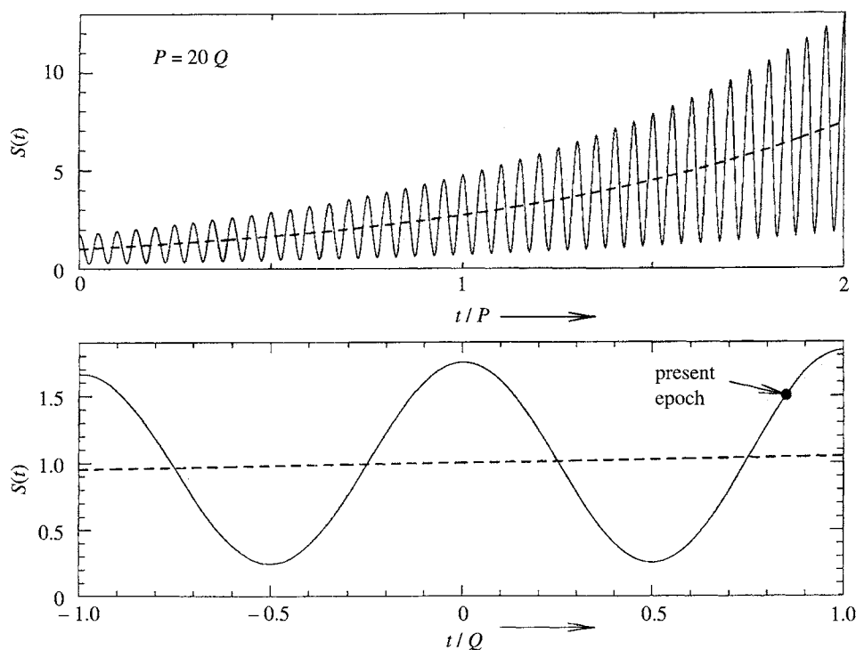
Figure 1. The scale factor S(t) of the QSSC plotted (in the upper half of the figure) against t to show how several oscillatory cycles of short period Q are accommodated in the longer e -folding time P of the exponential expansion. Here P = 20Q and (in the lower half of the figure) we see a few oscillations on an expanded timescale with our present epoch marked.
