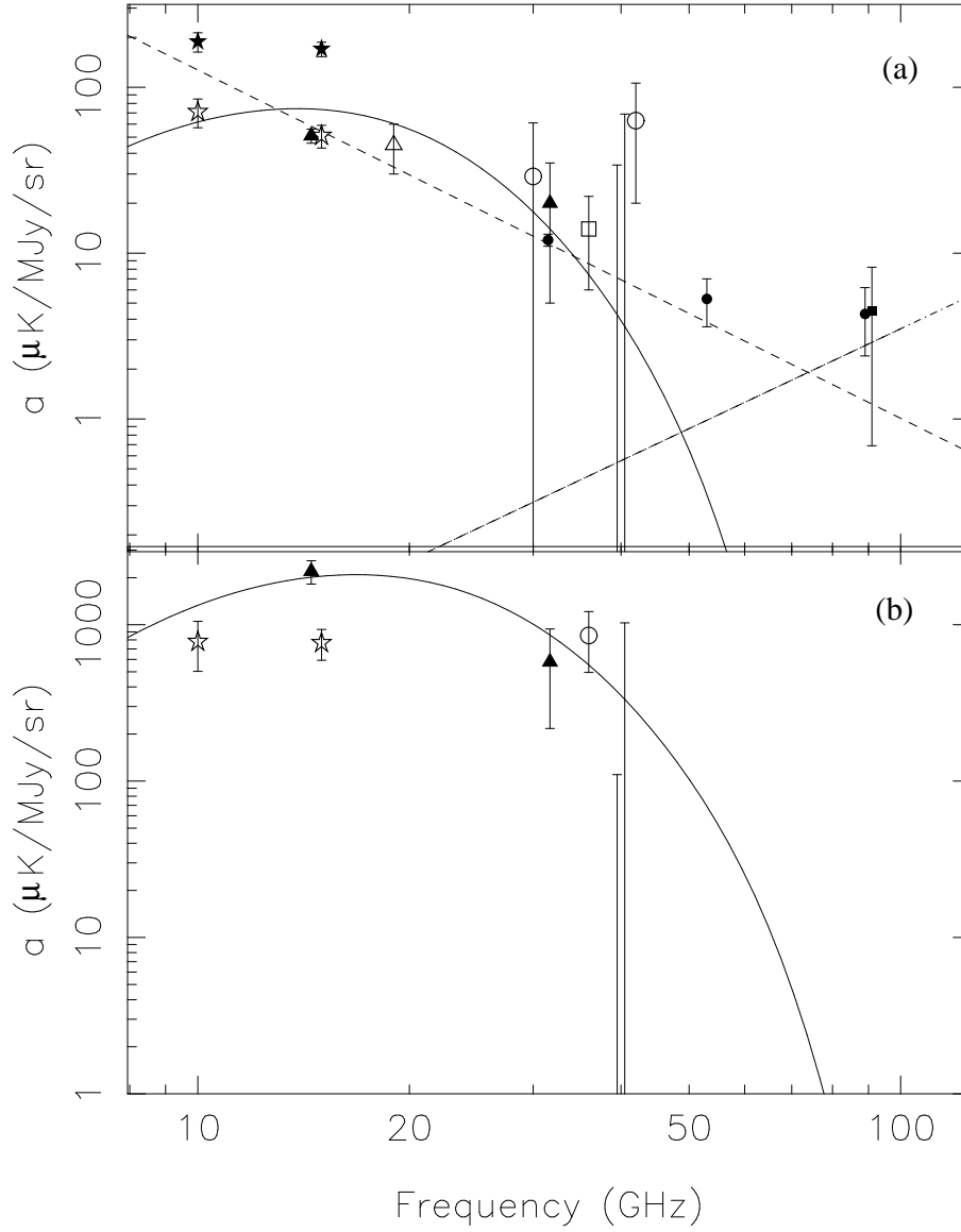
Fig. 1.— a ) Correlation slopes between CMB anisotropy data and the dust 100\ \mu\text{m} template. Two standard deviation upper limits obtained for PyV from analysing all the fields and from analysing the SP94 overlap region only are both shown at \sim 40 GHz. b ) Correlations with the 12\ \mu\text{m} template. Results are also shown for other experiments: Tenerife (open stars, de Oliveira-Costa et al. 2001; filled stars, Mukherjee et al. 2001), OVRO (filled triangles), 19GHz (open triangles), SP94 (open circles), Saskatoon (open square), Boomerang (filled rectangle), and DMR (filled circles). The solid curves are representative of a spinning dust spectrum, the dashed and the dot-dashed lines represent free-free and vibrational dust emission spectra, respectively.
