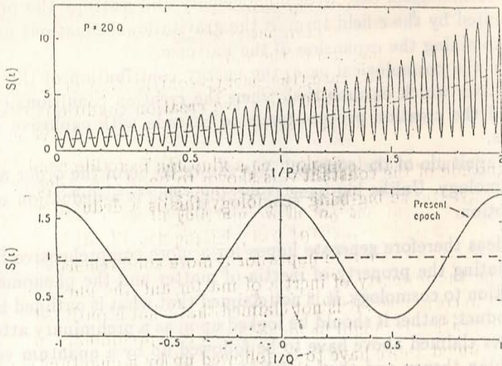
Figure 1. S(t) plotted against t/P (upper panel) and against t/Q (lower panel).
