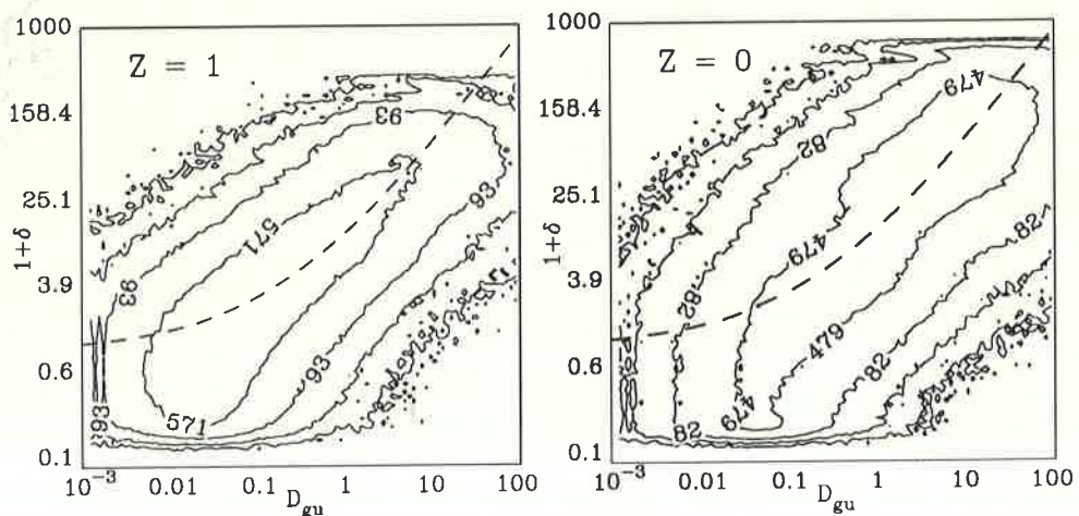
Figure 1. Contours of equal population on D_{gu} - (1 + \delta) plane. These have been drawn for CDM at Z = 1, 0 . Dashed line shows the relation for spherical top hat collapse.
