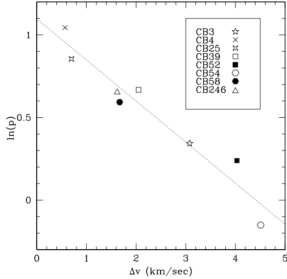
Figure 2. The log of average of observed polarization \ln(p) is plotted against the turbulence \Delta v ( \text{km s}^{-1} ) for various clouds. The line of best fit \ln(p) = 1.0831 - 0.2424\Delta v is shown.
