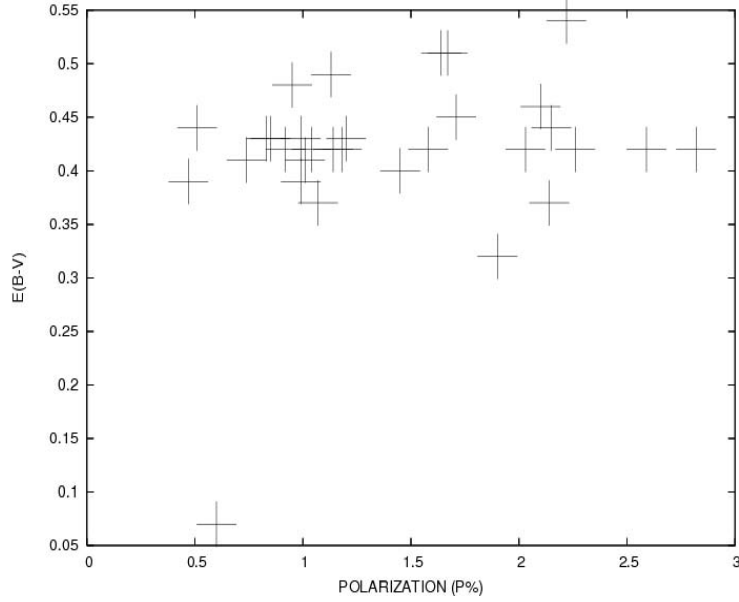
Figure 3. The polarization values observed for individual stars in the cloud CB3 are plotted against the corresponding colour excess E(B - V) values. The error values in polarization are typically less than 0.5 per cent (Sen et al. 2000).
