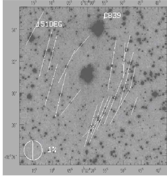
Figure 1. A map showing background star polarization for a typical cloud CB39, taken from Sen et al. (2000).
