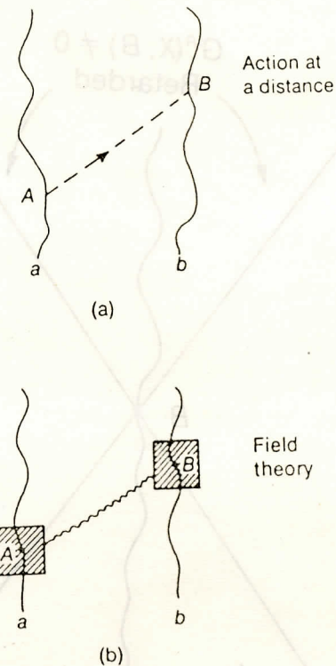
FIGURE 3 : (a) In the action-at-a-distance picture the influence from the point A on the world line of particle a is transmitted directly across spacetime (along the dotted track) to the point B on the world line of particle b . (b) In field theory the field in the neighborhood of A (shown by the shaded region) is disturbed: the disturbance propagates across spacetime as a wave in the ambient field and reaches the neighborhood of B . The disturbance then exerts a force on b at B . This is how the influence propagates from a to b .
