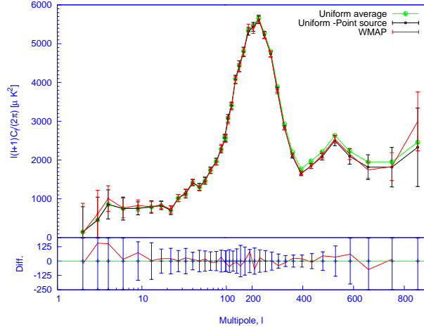
Figure 1: The angular power spectrum estimated from the WMAP multi-frequency using a self-contained model free approach to foreground removal [2] (black curve) is compared to the WMAP team estimate (red). The published binned WMAP power spectrum plotted in red line with error bars for comparison. The lower panel shows the difference in the estimated power spectra. The method holds great promise for CMB polarization where modeling uncertainties for foregrounds are much higher.
