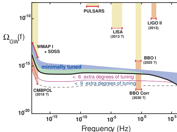
Figure 2: The figure taken from shows the theoretical predictions and observational constraints on primordial gravitational waves from inflation. The gravitational wave energy density per logarithmic frequency interval, (in units of the critical density) is plotted versus frequency. The blue region represents the range predicted for simple inflation models with the minimal number of parameters and tunings. The dashed curves have lower values of tensor contribution, r , that is possible with more fine tuned inflationary scenarios. The currently existing experimental constraints shown are due to: big bang nucleosynthesis (BBN), binary pulsars, and WMAP-1 (first year) with SDSS. Also shown are the projections for LIGO (both LIGO-I, after one year running, and LIGO-II); LISA; and BBO (both initial sensitivity, BBO-I, and after cross-correlating receivers, BBO-Corr). Also seen the projected sensitivity of a future space mission for CMB polarization (CMBPol).
