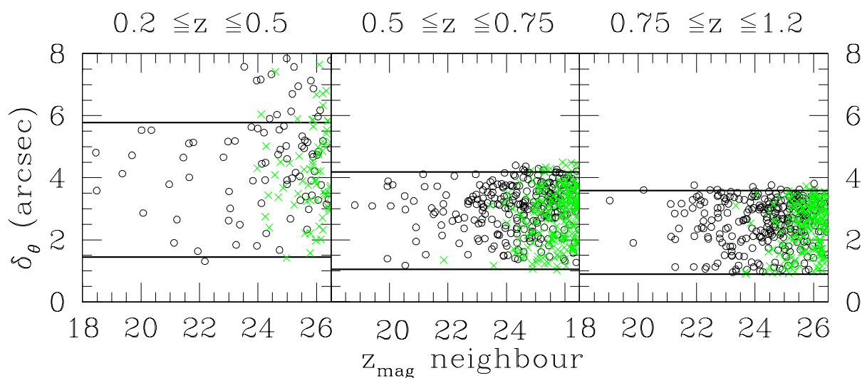
Fig. 7.— The angular separation between the main galaxy and the neighbour identified in the z filter Vs the z magnitude of the neighbour, segregated into three redshift bins as indicated. The open circles are neighbours which have measured K_s magnitude, whereas the green crosses are neighbours which do not have K_s magnitude. The horizontal lines correspond to 20h_{100}^{-1} kpc and 5h_{100}^{-1} kpc at the mean redshift of each bin.
