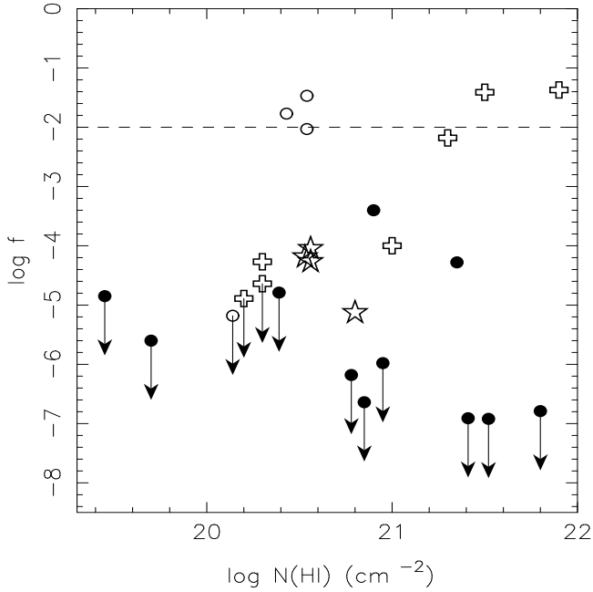
Fig. 3. Molecular fraction, f = 2N(\text{H}_2)/(2N(\text{H}_2)+N(\text{H I})) , versus H I column density. Damped Lyman- \alpha systems observed at high spectral resolution are indicated by filled circles (verticle arrows are for upper limits). Measurements in the Magellanic clouds by Richter (2000) are indicated by open crosses. Open circles and open stars are for, respectively, lines of sight perpendicular to the disk of our Galaxy and lines of sight toward the Magellanic clouds (Shull et al. 2000). The horizontal dashed line marks the transition from low to high molecular fraction in the local Galactic gas ( f = 0.01 ; Savage et al. 1977).
