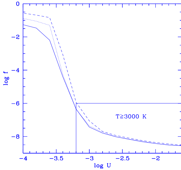
Fig. 5. Molecular fraction versus ionization parameter ( U = n_{\text{phot}}/n_{\text{H}} ) through a plane parallel slab with \log N(\text{H I}) = 21 , metallicity 0.03 solar, dust to metal ratios 0.3 (dashed), 0.1 (dotted) and 0.03 (solid) that in our Galaxy, illuminated by a starburst-like spectrum. The models with \log f < -6 have \log U > -3.2 and T > 3000 K.
