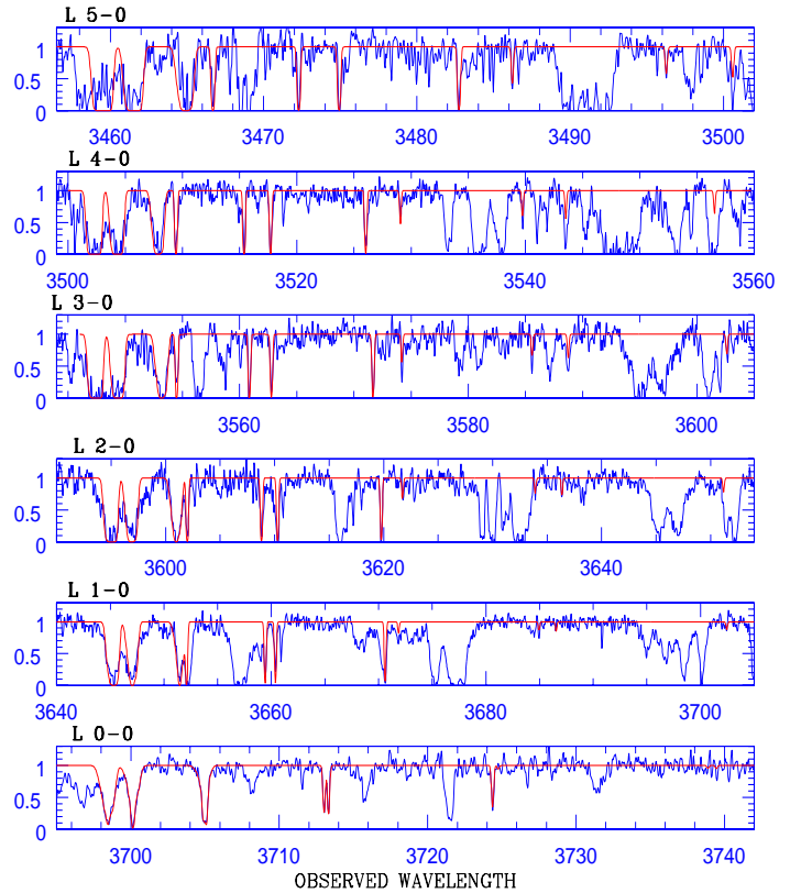
Fig. 1. Portions of the PKS 1232+082 normalized spectra. Fit models for \text{H}_2 absorption lines at z_{\text{abs}} = 2.3377 are over-plotted.
