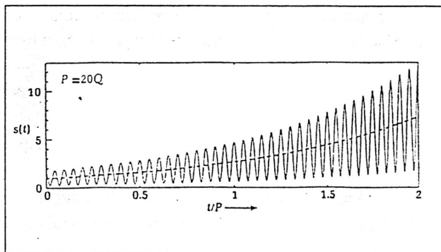
Figure 3 The Quasi-Steady State Cosmology shows expansion over a long time scale with cycles of expansion and contraction. This universe did not have any finite epoch of origin but has been in existence perpetually.
