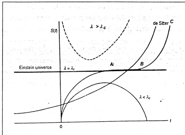
Figure 2 The scale factors of some of the different types of models with a non-zero cosmological constant are shown. In a typical model, by choosing \lambda close to the critical value \lambda_c , we can have a universe which expands from 0 to A, stays nearly static over an arbitrarily long stretch from A to B and then expands from B to the present C. Note that over the stretch BC the Universal expansion tends to accelerate. The figure also shows the 1917 models of Einstein and deSitter.
