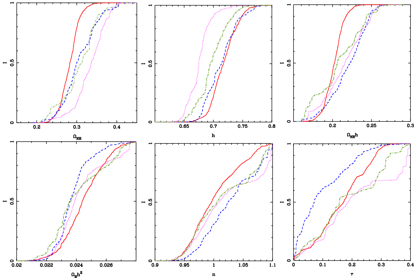
FIG. 7 (color online). Panels for \Omega_{\text{NR}} , h , \Gamma = \Omega_{\text{NR}}h , \Omega_b h^2 , n , and \tau . Solid curve is for \Lambda\text{CDM} , dashed curve for models with constant w , dotted-dashed for p = 1 , and dotted curve for p = 2 .
