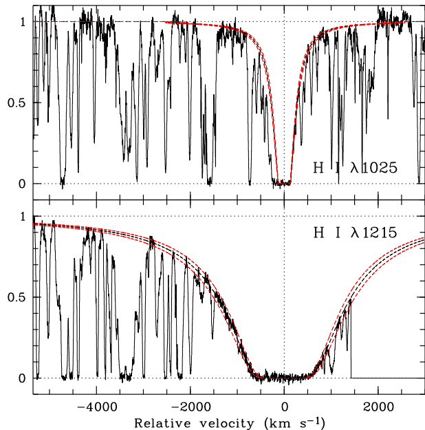
Figure 3. Portions of the normalized UVES spectrum showing the damped Ly \alpha and Ly \beta lines of the DLA system at z_{\text{abs}} = 3.025 toward Q0347–383. The best-fitted Voigt profiles superimposed on the data correspond to N(\text{H I}) = (3.6 \pm 0.4) \times 10^{20} \text{ cm}^{-2} .
