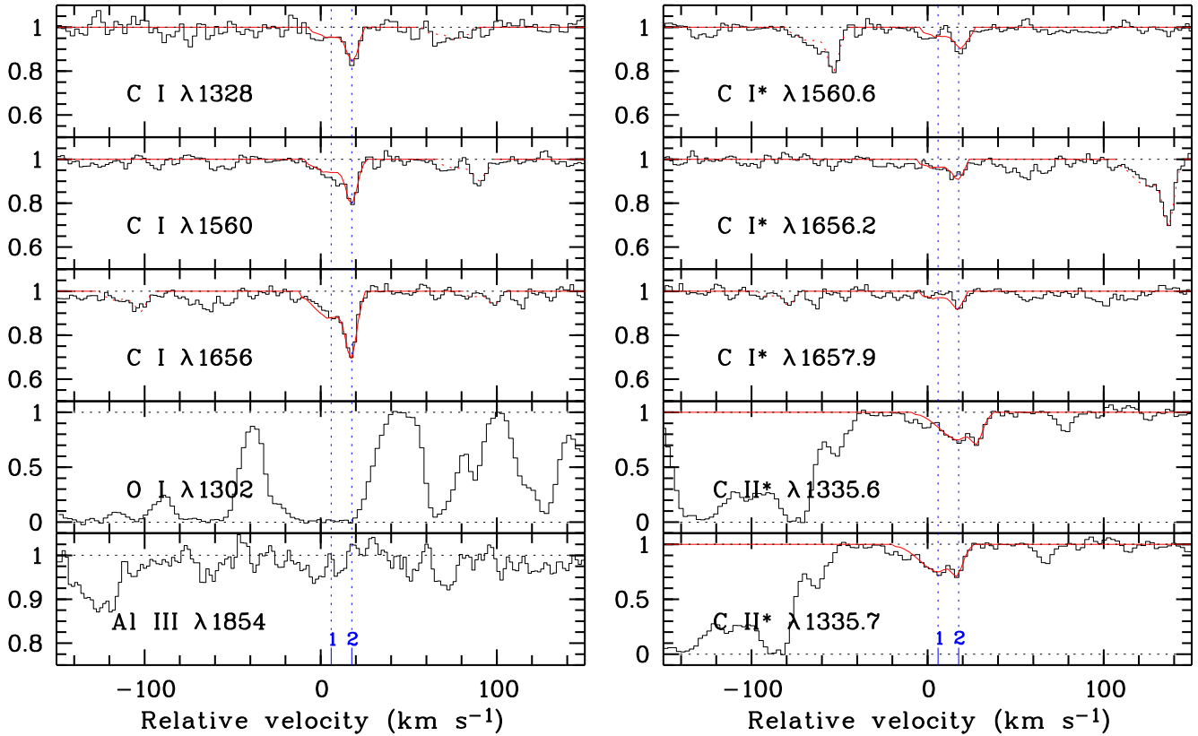
Figure 9. Absorption lines from the ground-state of C I (upper part of left panel) and fine-structure levels of C I and C II (right panels) at z_{\text{abs}} = 2.087 toward Q 1444+014. The two fitted components, where H 2 is detected, are indicated as in Fig. 8 by numbers in addition to vertical lines. The dotted parts in some of the synthetic profiles correspond to other transitions than the ones indicated. The origin of the velocity scale is the redshift of the main component as measured from the other metal lines ( z_{\text{abs}} = 2.08679 ). The redward shift of the C I components is apparent. The velocity profile of O I \lambda 1302 is shown for comparison. Note that Al III \lambda 1854 is barely detected (bottom part of left panel) in this sub-DLA system.
