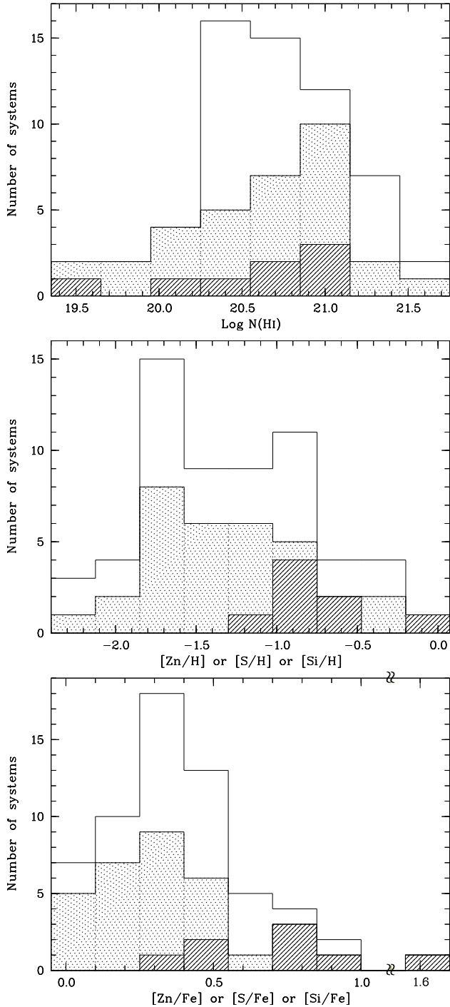
Figure 11. Distributions of neutral hydrogen column densities ( upper panel ), metallicities ( middle panel ; measured from either [Zn/H] , or [S/H] , or [Si/H] ) and depletion factors ( lower panel ; measured from either [Zn/Fe] , or [S/Fe] , or [Si/Fe] ) in, respectively, the global population of DLA/sub-DLA systems (overall distribution), our H_2 -survey sample (dotted histogram) and the sub-sample of H_2 -detected systems (hashed histogram).
