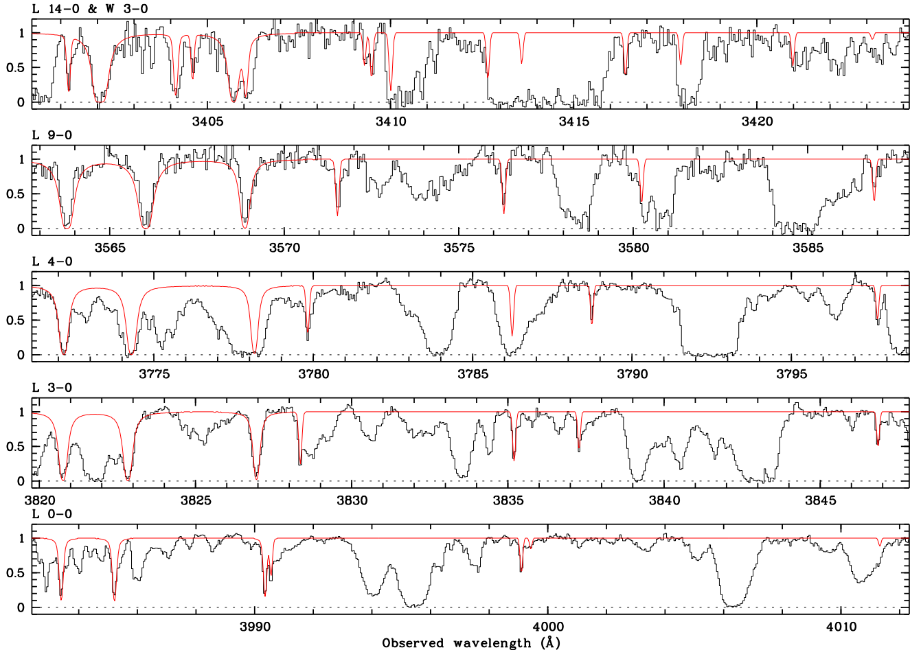
Figure 6. Voigt-profile fitting to the transition lines from the J = 0, 1, 2 and 3 rotational levels of the vibrational ground-state Lyman and Werner bands of H_2 at z_{\text{abs}} = 2.59471 toward Q0405–443. Only a few of the observed bands are displayed. H_2 is detected on this line of sight in a single gas cloud.
