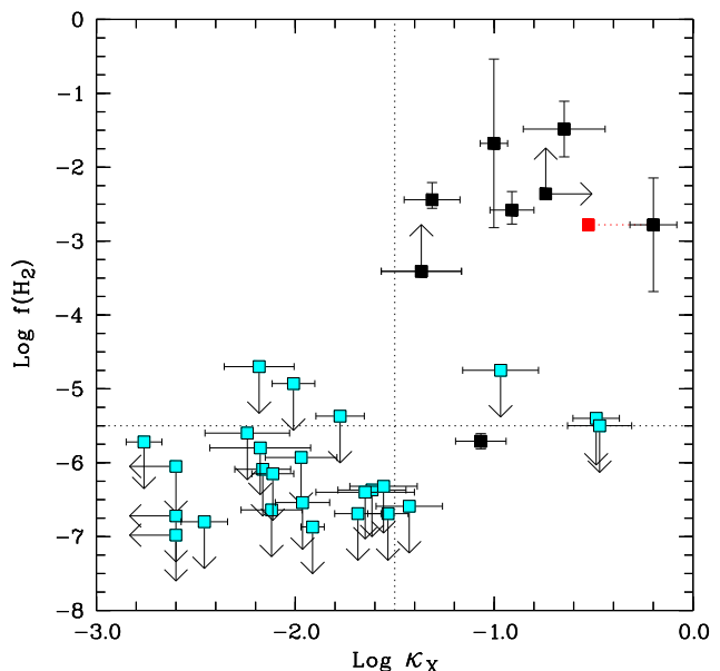
Figure 15. H_2 molecular fraction versus the amount of dust, or dust-to-gas ratio \kappa_X = 10^{[X/H]}(1 - 10^{[Fe/X]}) , with either X=Zn , or S , or Si . Drawing conventions are the same as in Fig. 14. A weak trend between the two quantities is apparent; however, several orders of magnitude spread in f(H_2) for a given dust content, among the detected cases, suggests that in addition to the amount of dust the physical conditions of the gas (density, temperature, UV flux) play an important role in governing the formation of H_2 in DLA systems.
