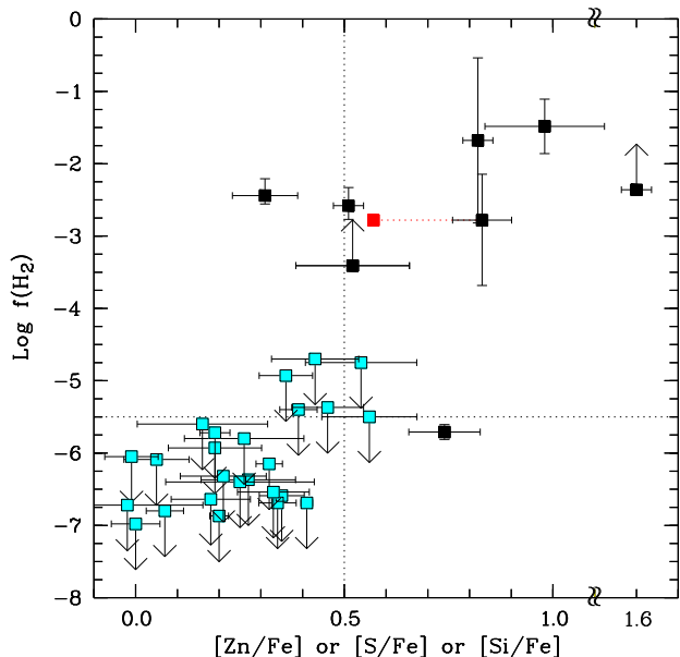
Figure 14. Mean H_2 molecular fraction versus depletion onto dust grains as estimated from the abundance of either X=Zn , or S , or Si relative to Fe , in the H_2 -survey sample (see Table 8). H_2 detections, measured by our group, are indicated by dark squares. The dotted line segment links data points for the DLA system toward Q 0551–366 considering either [Fe/Zn] or [Fe/S] . This is indeed the only one case where the difference between measured [X/Fe] ratios is significantly larger than 0.1 dex (i.e. 0.24 dex). The two dotted lines are drawn for illustrative purposes (see text).
