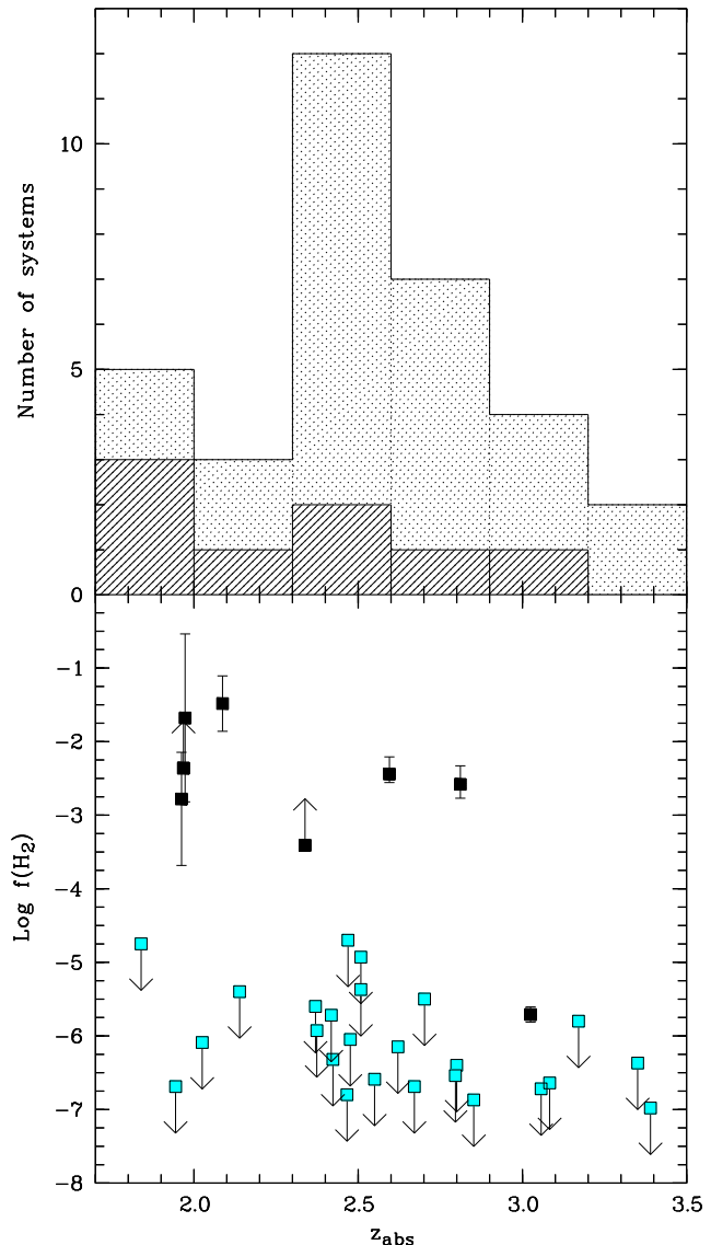
Figure 16. Upper panel: redshift distribution of the DLA/sub-DLA systems in our sample. The sub-sample of \text{H}_2 -detected systems is indicated by the hashed histogram. Lower panel: \text{H}_2 molecular fraction versus redshift. Detections are shown by dark squares and upper limits by shaded ones. Although the statistics are based on small numbers, the probability of finding molecules at z_{\text{abs}} \sim 2 is highest. This probably reveals that the amount of dust in DLA systems increases with time.
