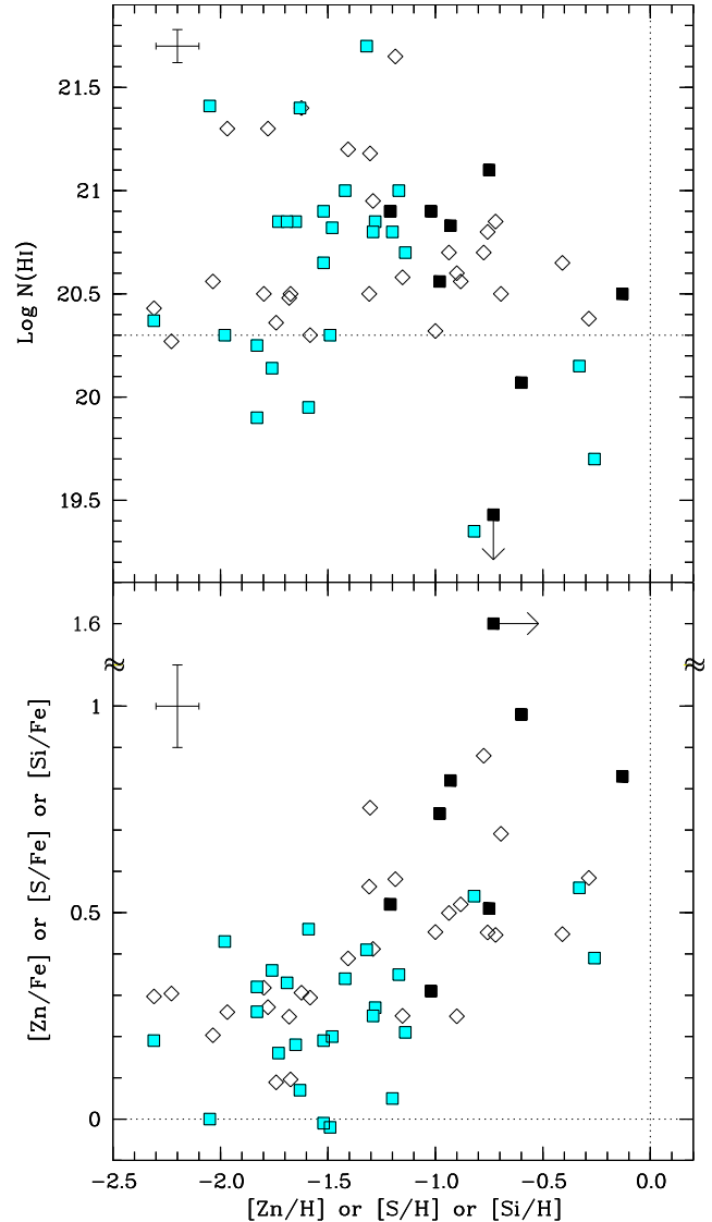
Figure 12. Neutral hydrogen column density ( upper plot ) and depletion factor ( lower plot ) versus metallicity in, respectively, the global population of DLA/sub-DLA systems (all symbols), our H_2 -survey sample (all squares) and the sub-sample of H_2 -detected systems (dark squares). The typical error bars are shown in the upper-left part of each plot. A correlation between metallicity and depletion factor is present at the 4\sigma significance level, confirming the trend previously detected by Ledoux et al. (2002a).
