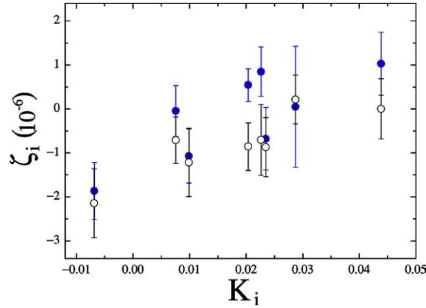
Fig. 1. The relative positions, \zeta_i = (z_i - \bar{z})/(1 + \bar{z}) , of lines that are seen in the spectra of both quasars Q 0405–443 (filled circles) and Q 0347–383 (open circles) are plotted versus the sensitivity coefficient K_i . Here, \bar{z} is the median redshift of all H_2 lines observed in one spectrum. The lines are L3R3, L3R2, L5R2, L6R3, L6P2, W0Q2, L8P3 and L12R3. The 1\sigma error bars shown are observational (without laboratory errors). They are of the order of 1 to 3 mÅ (in the observer's frame). It can be seen that both sets of measurements are mutually consistent within observational errors. The fact that the two independent observational measurements agree well suggests that our data calibration and measurement procedure are reliable at the level required for the study.
