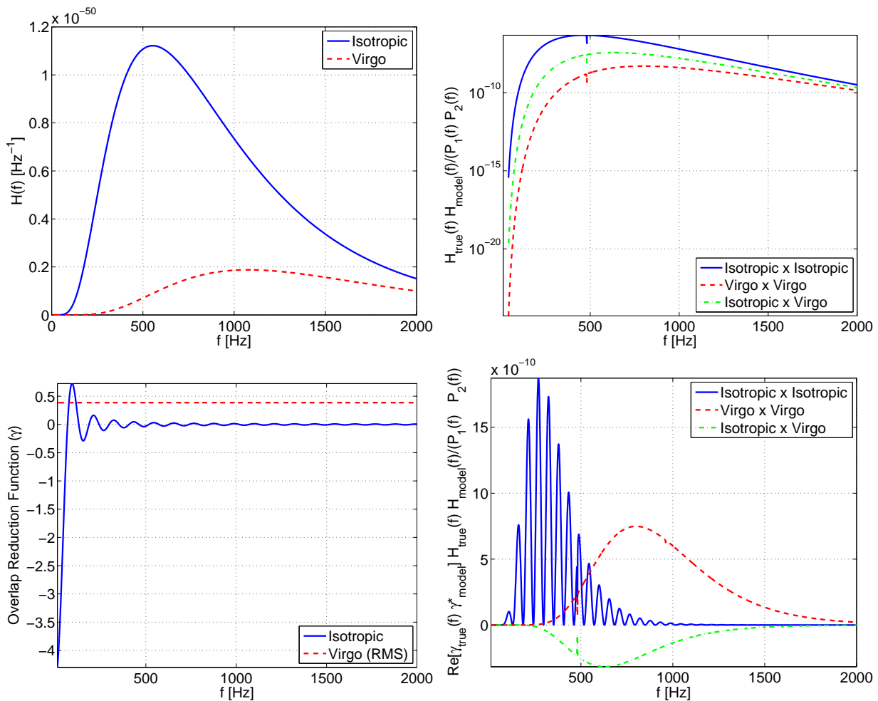
FIG. 2: This figure shows how different quantities combine to yield small increases in the SNR for directed search for the Virgo cluster (dashed line) and isotropic search (solid line) with z_{\max} = 2 . Top left shows H(f) for isotropic background integrated over all sky and Virgo cluster; Top right the frequency spectrum part of the optimal search filter; Bottom left are the overlap reduction function. Bottom right is the final integrand in the expression for SNR, here the square-root of the ratio of the area covered under the solid line to that under the dashed line is the ratio of SNRs (in this case 0.7328) provided in Table II.
