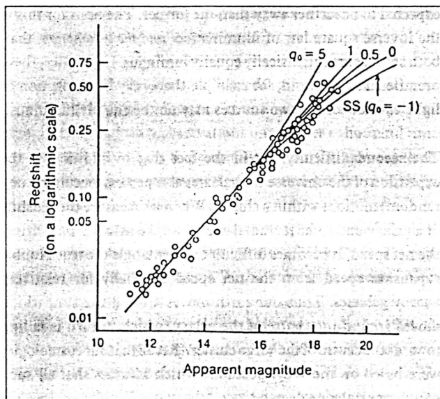
Figure 1 The redshift magnitude relation for first ranked cluster member galaxies. A number of theoretical curves are superposed on the data. These curves are labelled by a parameter q_0 , which measures the rate of slowing down of the expansion of the universe. It is called the deceleration parameter and its value for the flat Friedmann model is 0.5. We will refer to the steady state model in the final part of this series. (Based on J Kristian, A Sandage & J A Westphal, The Extension of the Hubble Diagram-III . The Astro-physical Journal , 221, 383 (1978).
