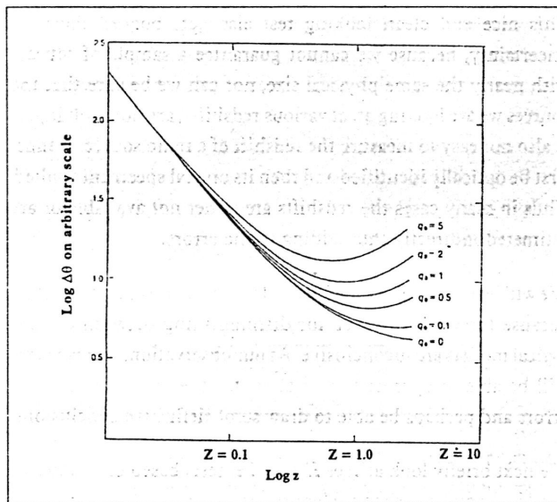
Figure 2 This figure illustrates how the angular diameter varies with redshift in a Friedmann model. Notice that at a specific redshift the angular diameter is the least in contrast to a Euclidean universe in which the angular diameter steadily decreases with distance. The label q_0 denotes the deceleration parameter as explained in the caption of the previous curve.
