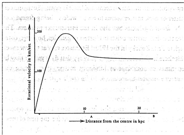
Figure 3 The typical flat rotation curve of a galaxy that indicates the presence of dark matter.
