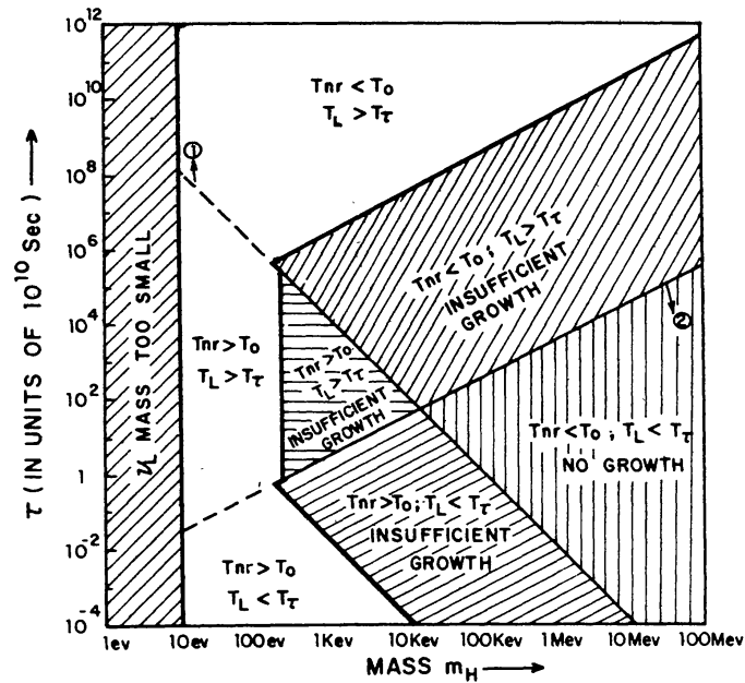
Figure 2. Lifetime \tau is plotted against mass m_H . Line (1) distinguishes case (a) from case (b) while line (2) separates the region T_L > T(\tau) from T_L < T(\tau) . The thick line separates the allowed regions (from growth of fluctuation analysis) from the 'not allowed' regions. For case (a) with T_L > T(\tau) the only constraint is that m_H < 173 eV, while for T_L < T(\tau) growth is sufficient only for regions to the left of the line given by Equation (29) (see text). For case (b), T_L < T(\tau) has no provision for growth to occur at any time (region below line). For T_L > T(\tau) growth is sufficient only for regions above the line given by Equation (38).
