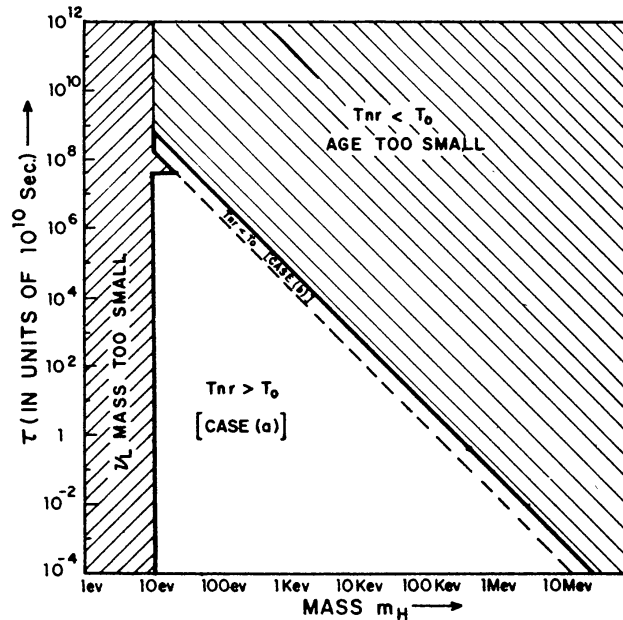
Figure 1. The lifetime \tau (in units of 10^{10} s) is plotted against the mass of the heavy neutrino, m_H . The broken line separates the two cases (a) and (b) (see text). For the case (a), the regions above the horizontal line at \tau \simeq 10^{17} s are not allowed from the constraint that \tau is less than the age of the universe. For case (b) this constraint is given by the thick line just above the broken line. In both the cases the regions which are not allowed are struck out.
