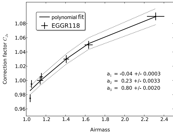
Fig. A.1. The plot shows the determined correction factors, C_{J_s} , of EGGR118 over the corresponding airmasses and the fit to the data points, a polynomial of the 2nd degree. The coefficients of the polynomial are given by the a_i , beginning with the leading coefficient.
