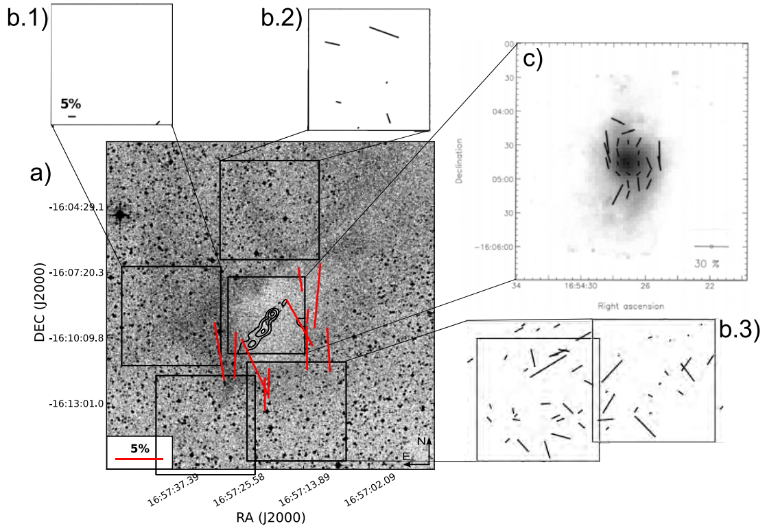
Fig. 2. CB68 - a ) DSS-map with overlaid near-IR polarization vectors observed with ISAAC/VLT. The length of the vectors shows the degree of polarization, and the direction gives the position angle. Only vectors with P/\sigma_P > 3 are plotted. The contour lines represent the ^{12}\text{CO}(3-2) spectral channel maps obtained with the JCMT. The black contour lines give the blueshifted (south-eastern), the grey, dotted contour lines give the redshifted (north-western) outflow lobe. Contour levels at 0.25, 0.50, 0.75, ... K (from Vallée et al. 2000, HPBW of 14'' ; reproduced by permission of the AAS). b.1-3 ) Same as a ) but with polarization vectors obtained with IFOSC/IGO in the optical. c ) Intensity map overlaid with polarization vectors obtained with SCUBA/JCMT in the sub-mm (Vallée et al. 2003, reproduced by permission of the AAS).
