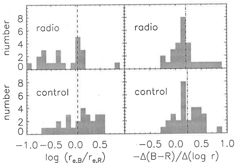
Fig. 2.— The distribution of r_e(B)/r_e(R) (left) and the color gradient (right) for the radio and control samples. Negative numbers on the x-axis are indicative of galaxies with excess blue emission towards the center.
