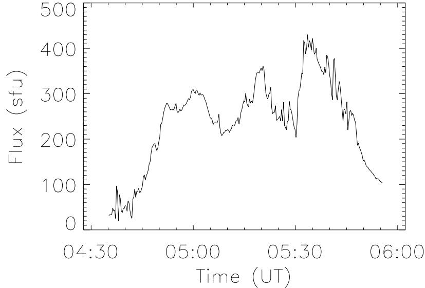
Figure 8. The 1060 MHz lightcurve from GMRT observations. The three peaks are clearly evident. The first onset of nonthermal emission at this frequency occurs at 04:48 UT. The peak of this lightcurve is normalized with respect to the peak of the 1 GHz lightcurve from the NoRP ( http://solar.nro.nao.ac.jp/norp/html/daily/ ). Figure 6 shows 16 s snapshot images near the three peaks of this lightcurve.
