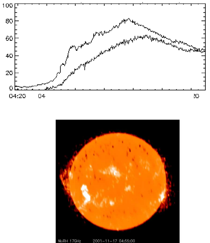
Figure 3. Upper panel: The upper curve is the 17 GHz lightcurve and the lower curve is the 34 GHz lightcurve from the NoRH. The vertical axis gives the flux in SFU. Both the lightcurves show a gradual rise and decay, implying that the radiation at these frequencies is thermal in nature. This radiation arises primarily from the active region situated at S18E40, that is evident in the lower panel. Lower panel: Image of the Sun at 17 GHz at 04:55 on Nov 17 2001 from the NoRH showing the erupting prominence on the east limb. The prominence, which was situated towards the northeast of the thermal active region emission evident at S18E40, erupted at \sim 04:48 UT. A movie of this event is available at http://solar.nro.nao.ac.jp/norh/html/10min/
