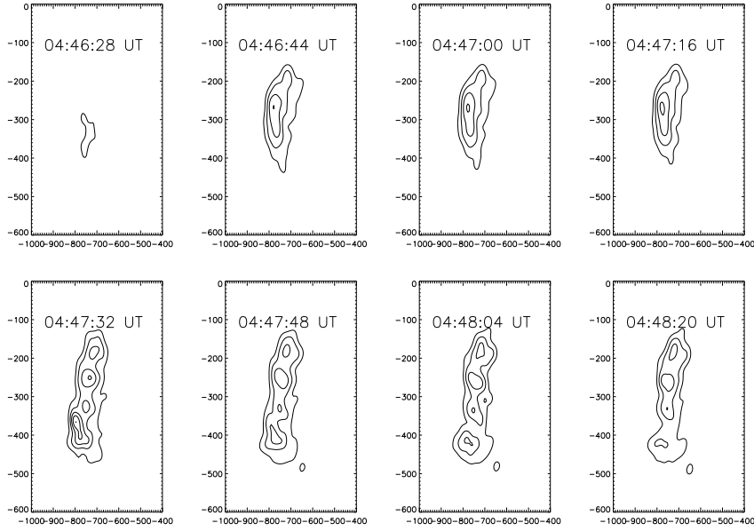
Figure 10. Snapshots at 16 second intervals near the rising edge of the first peak in the GMRT light curve. The contour levels and restoring beam are the same as those in figure 9. It is clearly evident that the first peak of the 1060 MHz emission occurs between 04:47:32 and 04:47:48 UT.
