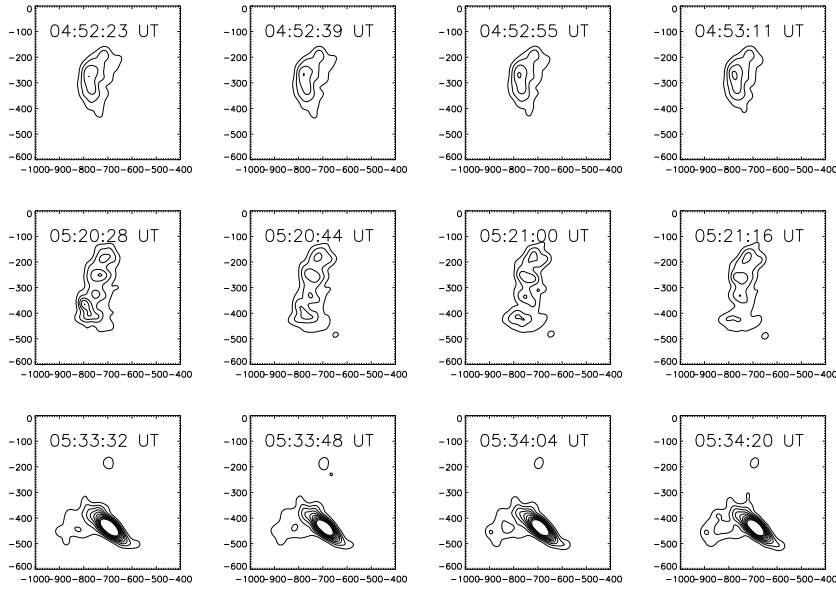
Figure 9. Contours of 16 s snapshots of the GMRT 1060 MHz emission. The center of these images is at S15E46 and the field of view is 500'' \times 500'' . The restoring beam is 34'' \times 24'' . The contour levels are 0.1, 0.2, 0.3, 0.4, 0.5, 0.6, 0.7, 0.8, 0.9 and 1.0 times the flux at the largest peak, which occurs at 05:33 UT. We show four sets of 16 s snapshots starting at 04:52:23 UT, 05:20:28 UT and 05:33:32 UT. These correspond to the three peaks of the 1060 MHz lightcurve (figure 8). The emission at the peaks of 04:52 UT and 05:20 UT are from a NS oriented loop system, whereas the emission at the peak at 05:33 UT is from a NE-SW oriented loop. The brightness temperature of the emission at each of these peaks is \lesssim 10^8 K.
