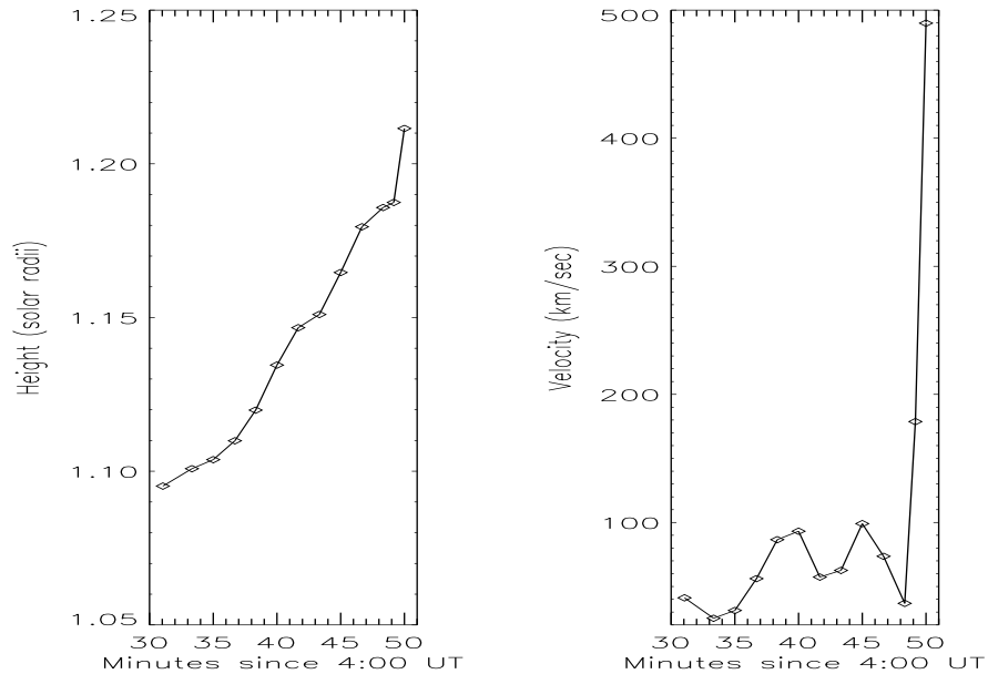
Figure 5. Left panel: The height-time profile of the lower envelope of the drifting continuum evident in the dynamic spectrum of figure 4. It represents the upper end of a vertical current sheet that forms beneath the erupting prominence. Right panel: The velocity-time profile of the same feature. The abrupt increase in velocity at around 04:48 UT can be inferred from the increased curvature around this time of the lower envelope of the drifting continuum (figure 4).
