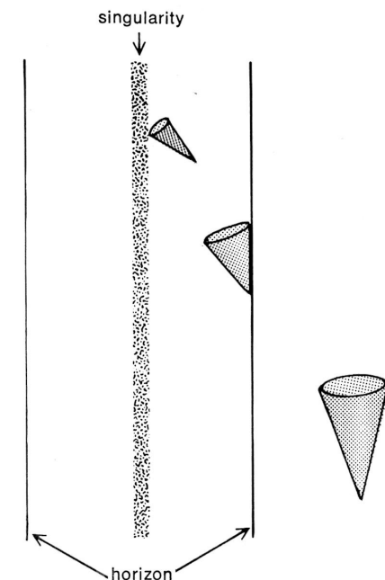
Figure 6. The light cones are oriented in this manner near a Schwarzschild black hole. Once inside the horizon all directions within the future light cone lead toward the central singularity.
