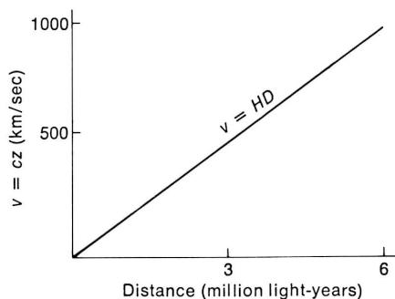
Figure 3. Hubble's original observations, which led to Hubble's law, extended to distances (as estimated by him) of the order of 6 million light-years, with redshifts corresponding to Doppler recession velocities of the order of 1000 km/sec. The distance scale has since been revised several times, and the present value of the Hubble constant is nearly 10–20% of Hubble's original estimate. (This range covers the present-day uncertainty of extragalactic distance estimates.)
