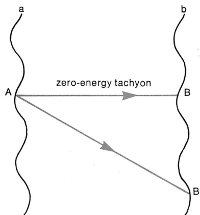
Figure 2. The zero-energy tachyon conveys momentum instantaneously from point A to point B on worldlines a and b . By the reinterpretation principle the tachyon along AB' traveling backward in time may be reinterpreted as having been emitted at B' and absorbed later at A.
