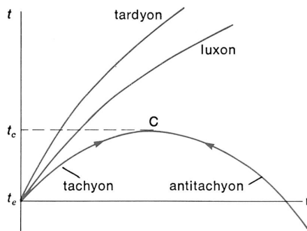
Figure 5. The trajectories of a tardyon, a luxon, and a tachyon emitted from the same space-time point are shown. The first two keep traveling forward in time, while the tachyon encounters a time barrier at C and turns back in time. By reinterpretation we may look upon C as the point of annihilation of a tachyon and an antitachyon.
