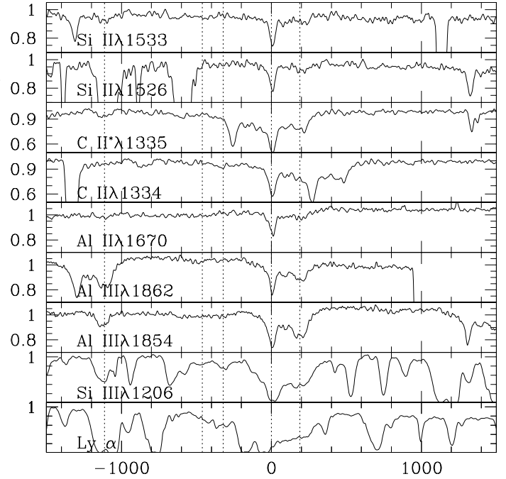
Fig. 6. Velocity plot of low ionization lines from the z_{\text{abs}} = 2.082 system. The vertical dotted lines mark some of the components discussed in the text. The main narrow component is at z_{\text{abs}} = 2.0819 .
