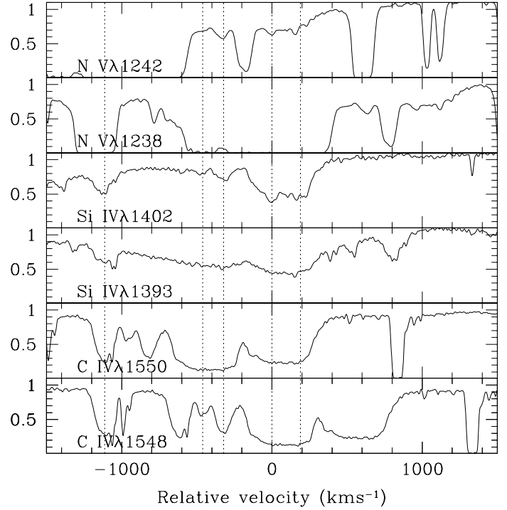
Fig. 5. Velocity plot of high ionization lines from the z_{\text{abs}} = 2.082 system. The vertical dotted lines mark some of the components discussed in the text.
