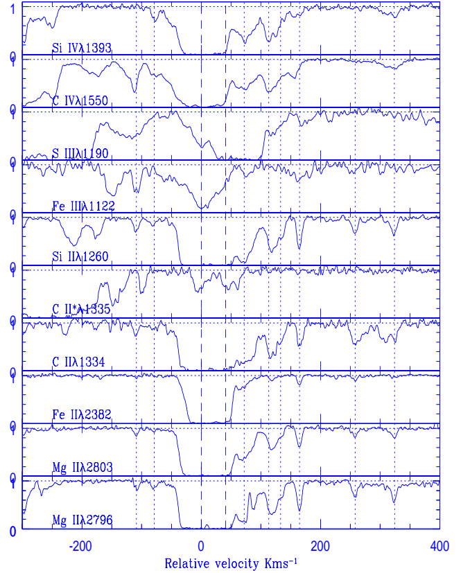
Fig. 14. Absorption profiles of some of the standard absorption lines in the z_{\text{abs}} = 2.139 system. The dotted lines show the position of the weak narrow components. The dashed lines show the position of low ionization components discussed in the text.
