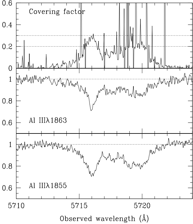
Fig. 8. Covering factor estimated from the Al III absorption at z_{\text{abs}} = 2.082 (top panel). Lower and middle panels give respectively the profiles of Al III \lambda 1855 and Al III \lambda 1863 (suitably shifted).
