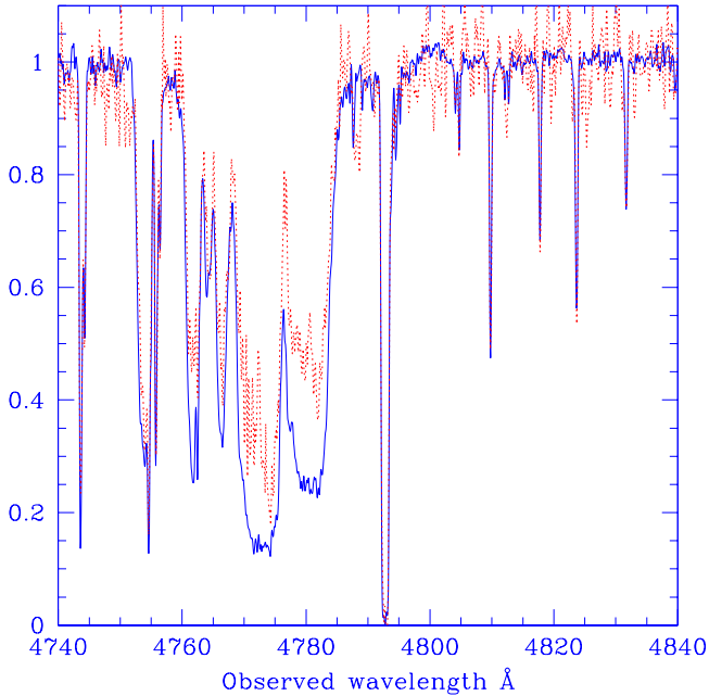
Fig. 10. Time variability of C IV absorption. The continuous line corresponds to our UVES data and the dotted line is the CASPEC spectrum from Lespine & Petitjean (1997). The resolution of the UVES spectrum is degraded to match that of the CASPEC data.
