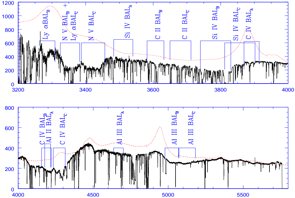
Fig. 1. Portion of the Tol 1037–2703 spectrum. A high-quality UVES spectrum of Q1101–264 shifted in wavelength and intensity is overlotted (dotted line). Position of various BALs discussed in the text are indicated. The subscripts ‘A’, ‘B’ and ‘C’ denote the z_{\text{abs}} = 1.51, 1.70 and 1.75 systems respectively.
