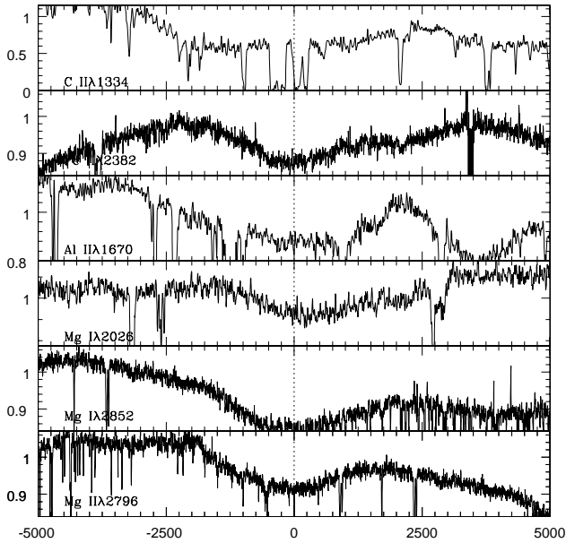
Fig. 3. Velocity plot of broad absorption lines from the z_{abs} = 1.5181 system.
