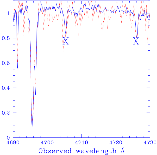
Fig. 11. Time variability of Si II absorption lines (marked with 'X'). The solid line corresponds to the UVES data and the dotted line is the CASPEC data from Lespine & Petitjean (1997).
