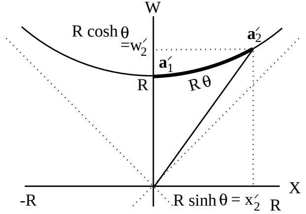
Figure 2. The 2-plane X - W for the case k = -1 , after the isometries f and g have been used to shift the two points \mathbf{a}_1 and \mathbf{a}_2 to \mathbf{a}'_1 and \mathbf{a}'_2 respectively, i.e. to (0, R) and (x'_2, w'_2) (resp.) in the X - W 2-plane. The hyperbola \mathcal{H}^1 in this plane is part of the 3-hyperboloid \mathcal{H}^3 defined by \langle \mathbf{a}, \mathbf{a} \rangle = R^2 . The inner product \langle \mathbf{a}'_1, \mathbf{a}'_2 \rangle evaluates to \langle \mathbf{a}'_1, \mathbf{a}'_2 \rangle = R w'_2 = R^2 \cosh \theta . The ‘arc-length’ R\theta (‘arc’ shown as extra-thick curve) is R\theta = R \cosh^{-1}(w'_2/R) .
