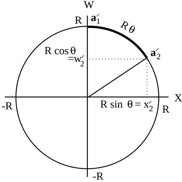
Figure 1. The 2-plane X - W for the case k = +1 , after the isometries f and g have been used to shift the two points \mathbf{a}_1 and \mathbf{a}_2 to \mathbf{a}'_1 and \mathbf{a}'_2 respectively, i.e. to (0, R) and (x'_2, w'_2) (resp.) in the X - W 2-plane. The circle \mathcal{S}^1 in this plane is part of the 3-sphere \mathcal{S}^3 defined by \langle \mathbf{a}, \mathbf{a} \rangle = R^2 . The inner product \langle \mathbf{a}'_1, \mathbf{a}'_2 \rangle evaluates to \langle \mathbf{a}'_1, \mathbf{a}'_2 \rangle = R w'_2 = R^2 \cos \theta . The arc-length R\theta (arc shown as extra-thick curve) is R\theta = R \cos^{-1}(w'_2/R) .
