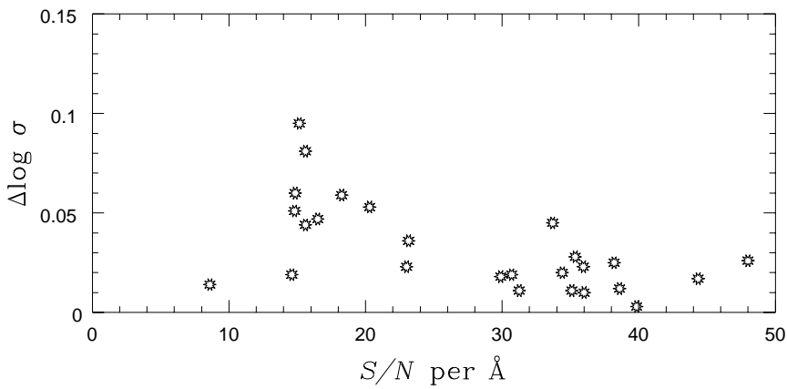
Fig. 8. The difference between results for velocity dispersions measured from repeat observations, plotted against the mean S/N per Å of each pair of spectra.
