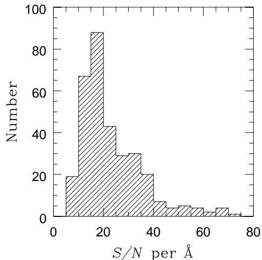
Fig. 1. The distribution of spectra as a function of the mean S/N per Å measured at the wavelength of Mgb.
