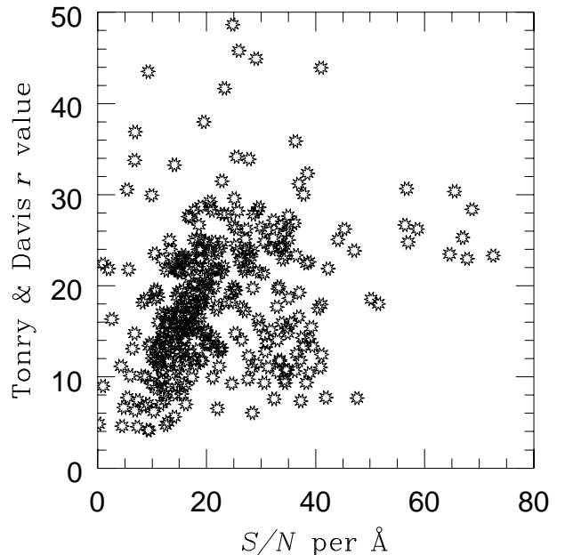
Fig. 3. A comparison of the S/N per Å of the spectra with the value of the Tonry & Davis r parameter from the cross-correlation, which is a measure of the ratio between the peak height and the noise, and is therefore an indicator of the accuracy of the results.
