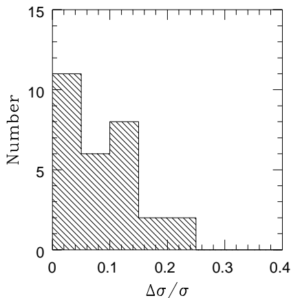
Fig. 9. Histogram of the fractional errors in the values of \sigma determined from repeat observations.
