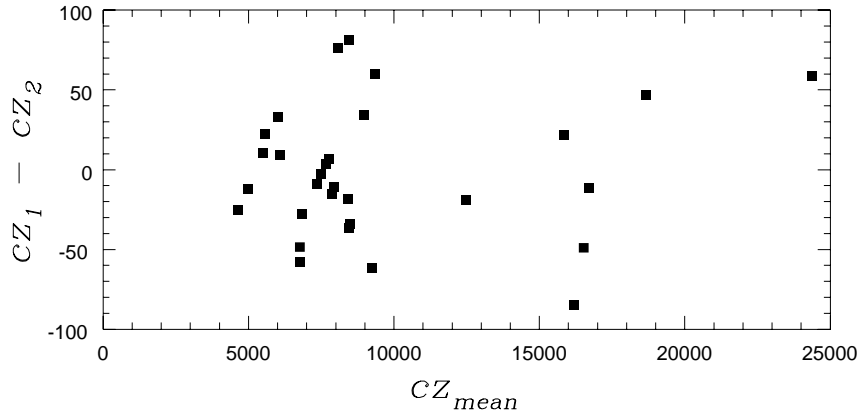
Fig. 6. Comparison of results for heliocentric radial velocity values determined from repeat observations.
