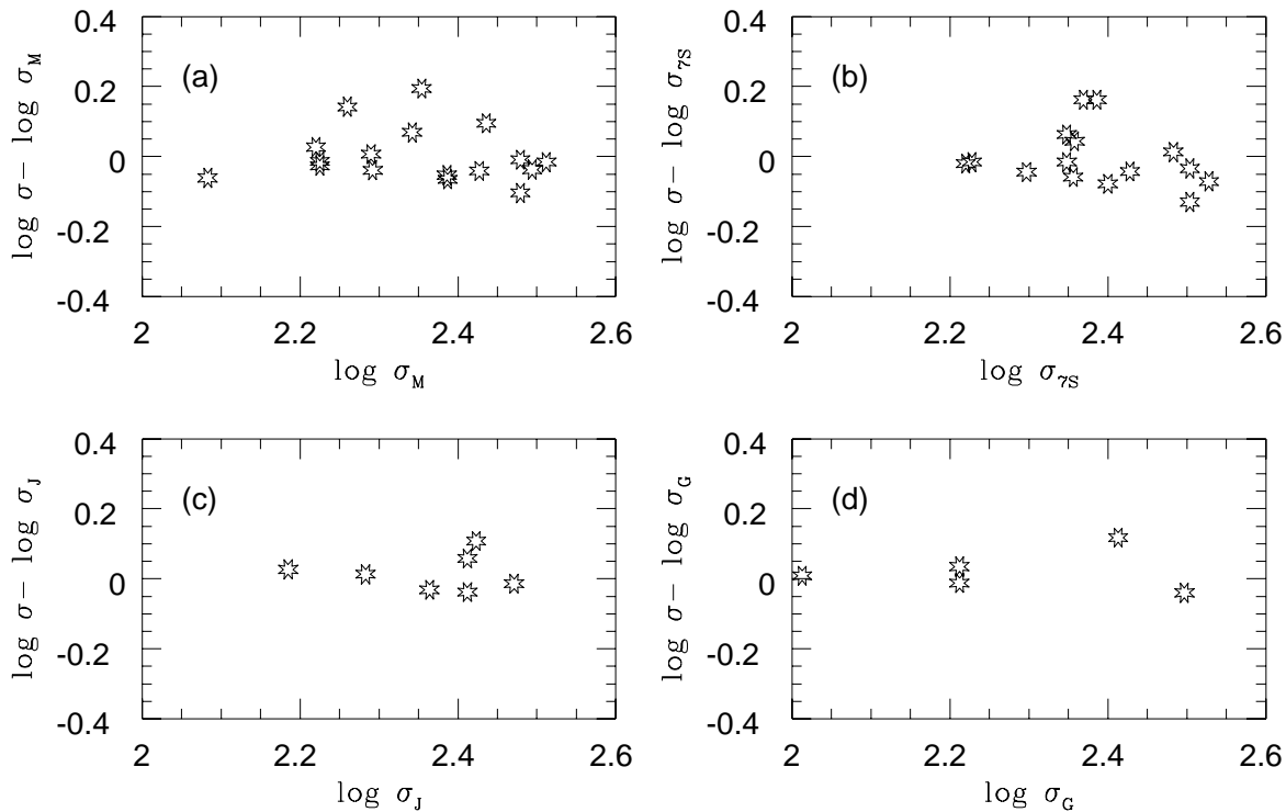
Fig. 12. Comparison of the results for velocity dispersions of standard galaxies with values from the literature: (a) McElroy (1995); (b) Davies et al. (1987); (c) Jørgensen et al. (1995); (d) González (1993).
