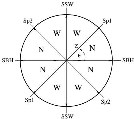
FIG. 1: The solution space showing different regions representing naked singularities, wormholes and black holes. Here \kappa = Z \sin \theta and \lambda = Z \cos \theta . N–Naked singularities, W–Wormholes, SBH–Schwarzschild black hole, SSW–Spatial Schwarzschild Wormhole, Sp1,2–Special solutions.
