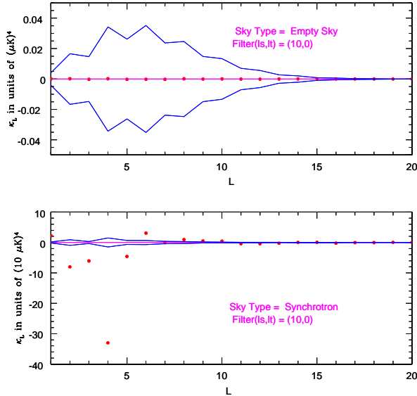
FIG. 1: CMB polarization maps with no foregrounds are statistically isotropic and have null bipolar power spectrum (top). Adding polarized synchrotron emission violates statistical isotropy and results in a detectable non-zero bipolar power spectrum (bottom). Red dots show the BiPS after bias subtraction and Blue lines show the 1 - \sigma of the cosmic variance.
