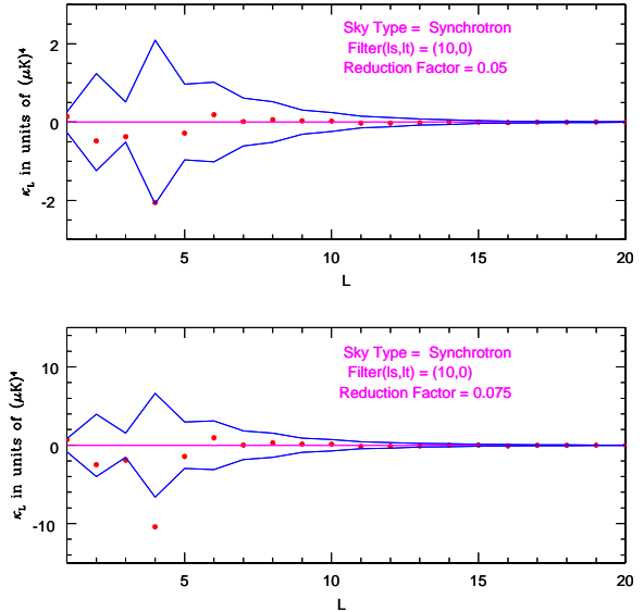
FIG. 2: Adding 5% of the polarized synchrotron emission just violates statistical isotropy (top). Adding 7.5% of the polarized synchrotron emission clearly violates statistical isotropy and results in a detectable non-zero bipolar power spectrum (bottom). Red dots show the BiPS after bias subtraction and Blue lines show the 1 - \sigma of the cosmic variance.
