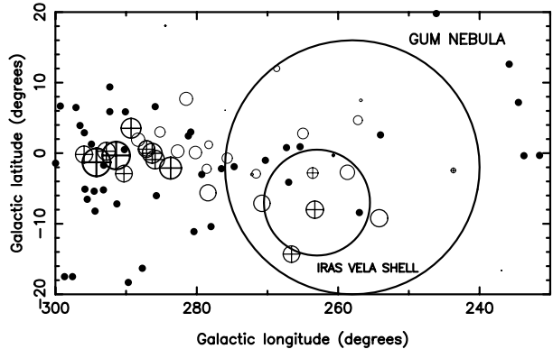
Fig. 1. Observed scatter broadening ( \tau_{sc} ) of pulsars at 327 MHz plotted as a function of the galactic coordinates. The circles with crosses correspond to pulsars for which earlier \tau_{sc} measurements are available. The open circles are the pulsars observed using the ORT. Size of these symbols is proportional to \log(\tau_{sc}) , where \tau_{sc} is in milliseconds. Pulsars indicated as “dots” are those for which the scatter broadening measurements are not available. The Gum nebula is indicated by the larger circle with radius of \sim 18^\circ with morphological center at l = 258^\circ and b = -2^\circ . The smaller circle indicates the IRAS-Vela shell, with a radius of \sim 7.5^\circ , with centre at l = 263^\circ and b = -7^\circ (adopted from Sahu 1992). Our sample consists also of pulsars outside the “main body” of the Gum Nebula (Chanot & Sivan 1983), as it is possible that the faint diffuse and filamentary extensions are possibly part of the nebula itself
