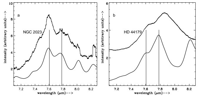
Fig. 7. PAH cations emission model in the 1200 to 1400\text{ cm}^{-1} region compared with observed spectra (a) PAHs with less than 40 C atoms in varying proportions (see text); (b) more than 40 C atoms (model III). The 7.7\text{ }\mu\text{m} band lies within the two vertical lines.
