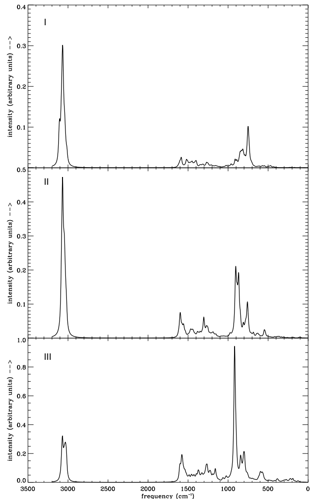
Fig. 2. Model spectra of co-added emissions from neutral PAHs with (I) less than 20 C atoms, (II) 20 to 40 C atoms, (III) more than 40 C atoms.
