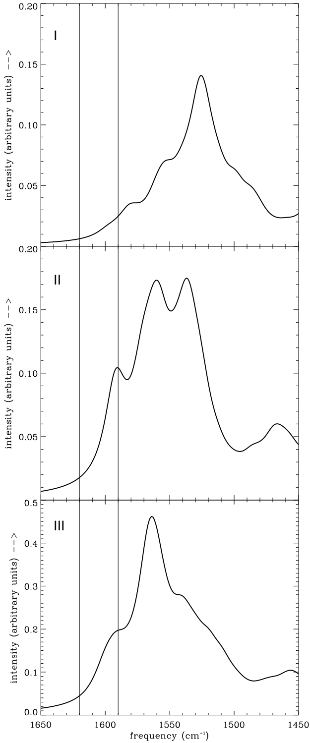
Fig. 5. Emission spectra of three cation models in the 1450 to 1650\text{ cm}^{-1} region. The observed 6.2\text{ }\mu\text{m} AIB lies within the two parallel lines.
