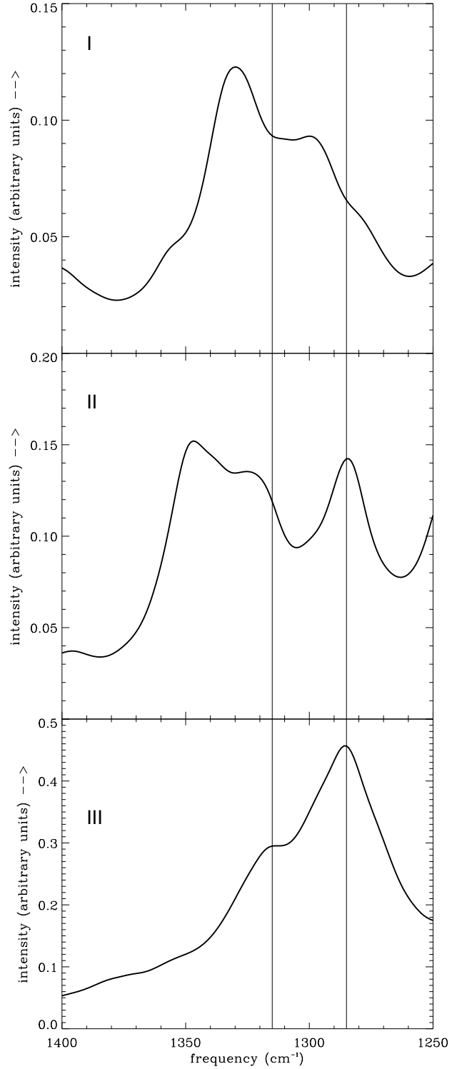
Fig. 4. Emission spectra of three cation models in the 1250 to 1400 cm^{-1} region. The observed 7.7 \mu m AIB lies within the two parallel lines.
