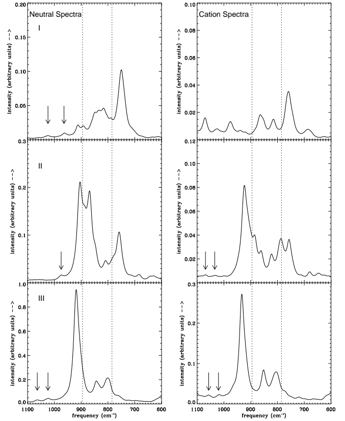
Fig. 6. Emission spectra of three models in the 600 to 1100\text{ cm}^{-1} region. Arrows point to blue outliers of 11.2\text{ }\mu\text{m} band. Dotted vertical lines represent central peak of 11.2 and 12.7\text{ }\mu\text{m} AIB.
