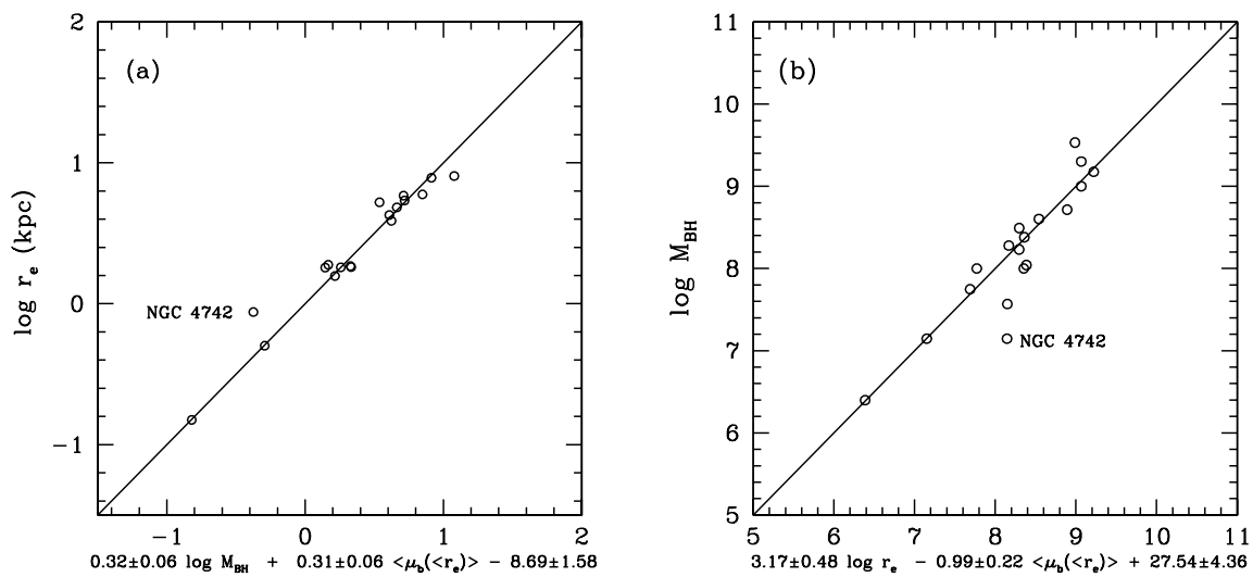
Fig. 1.— Edge-on views of the mass fundamental plane relations for nearby ellipticals: (a) along one of the shorter axes of the plane, \log r_e and (b) along another axis of the plane, \log M_{\text{BH}} .
