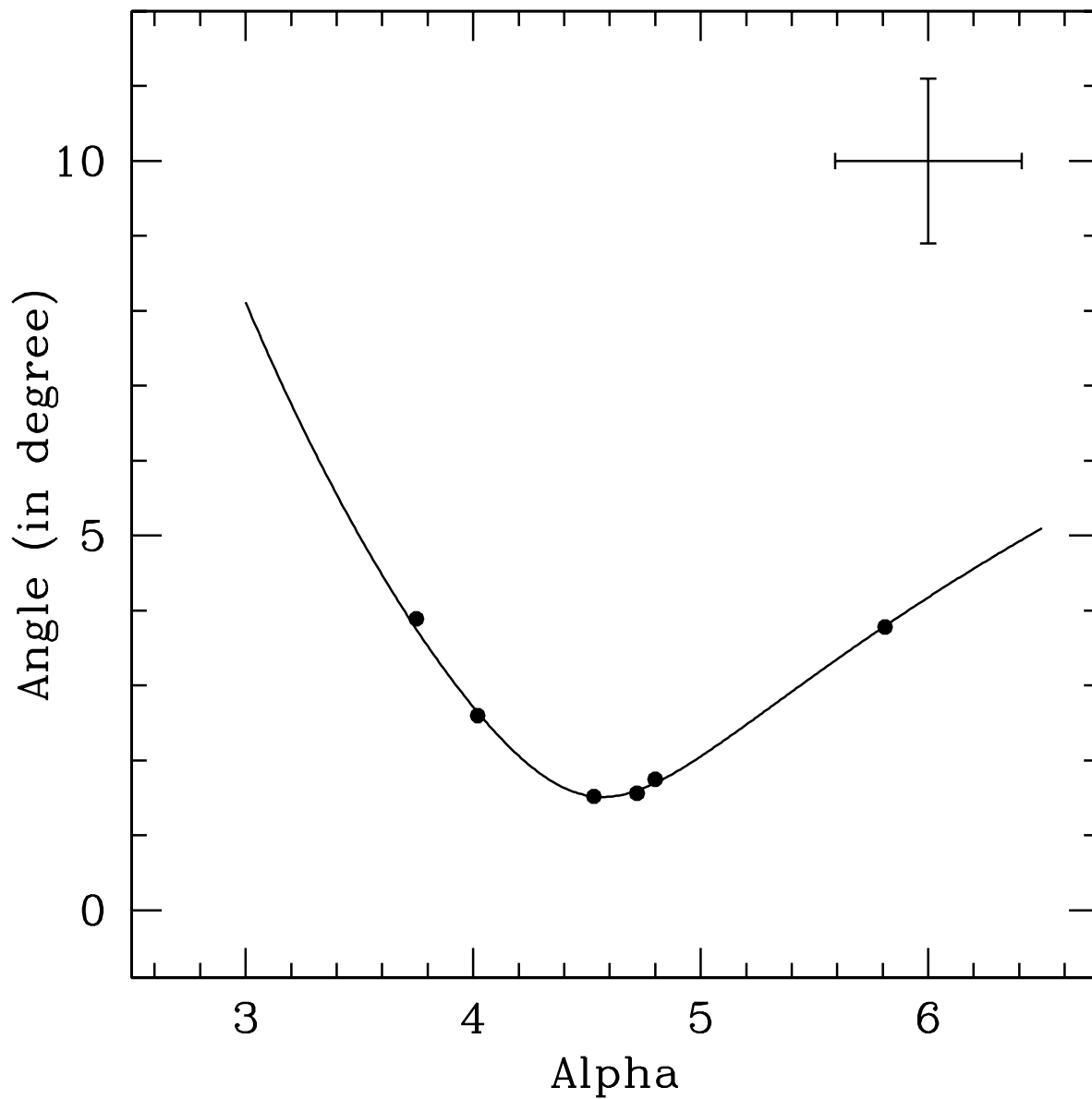
Fig. 2.— The curve shows the angle between (1) the best-fit mass FP, and (2) the plane derived using the fundamental plane in Equation 4 and the relation M_{\text{BH}} = \alpha \log \sigma + \beta for a range of values of \alpha . The filled circles indicate the angle for actual values of \alpha taken from the literature (see Tremain et al. 2002). The typical error in the measured values of \alpha and the derived angle between the planes is shown at the top right in the plot.
