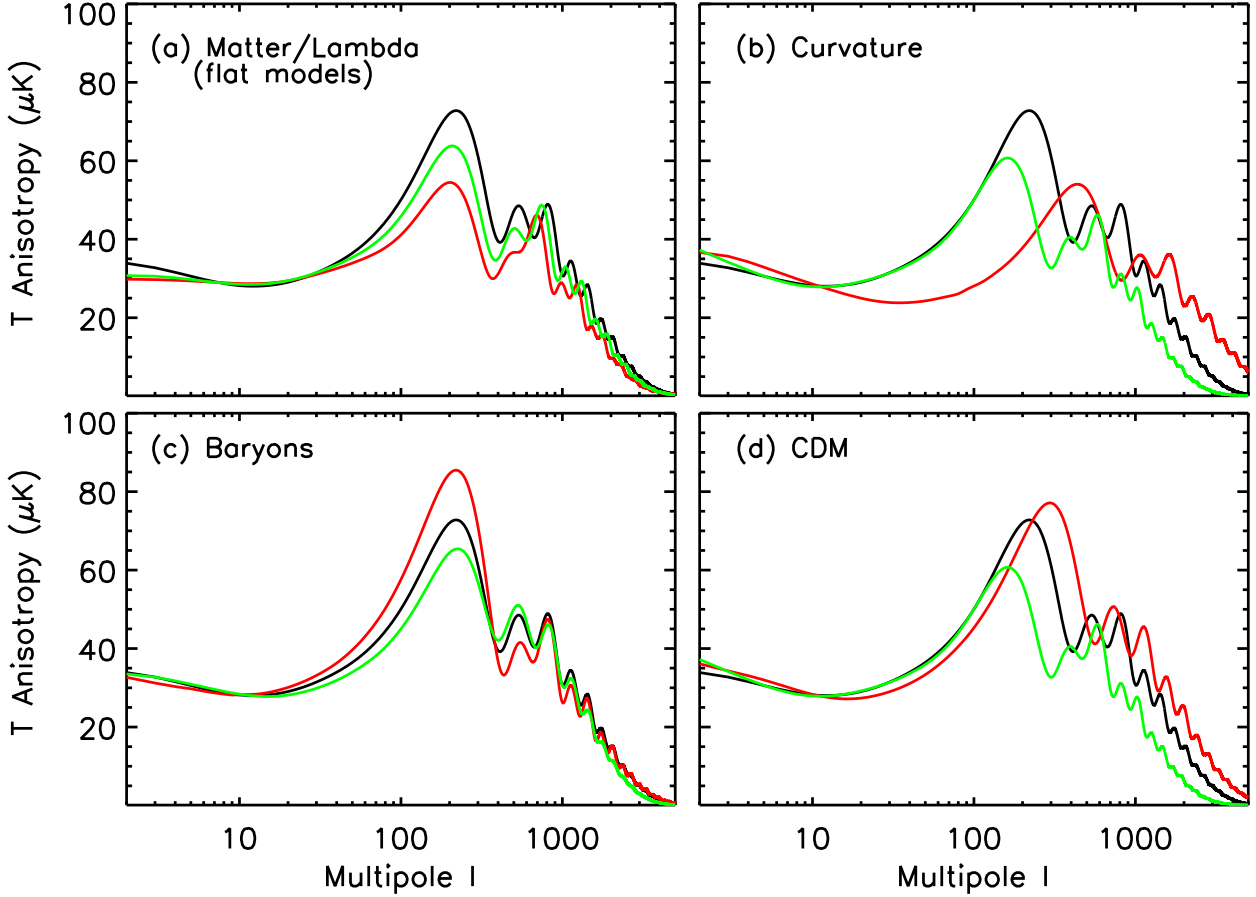
FIG. 2: The figure illustrates the sensitivity of the temperature anisotropy to changes in various parameters, about the standard \Lambda CDM model of Figure 1. The black (dark) line is always the standard \Lambda CDM model. Figure (a): Shows sensitivity to matter/lambda densities for flat models. The three plots with decreasing peak amplitudes result from increasing \Omega_m to 0.5 and 1, keeping total \Omega_T = 1 . Figure (b): Here the effect of total curvature on peak location is illustrated. The plot with the smallest l value for the first peak has \Omega_m = 0.448 , \Omega_\Lambda = 0.73 , while that with the largest is for an open universe, with \Omega_m = 0.27 and \Omega_\Lambda = 0 . Figure (c): Shows the sensitivity to the baryon density. For the three plots with decreasing first peak amplitudes, one has \Omega_b = 0.092 , 0.046 and 0.023 respectively. Figure (d): The sensitivity to the CDM density parameter. This is 0.112, 0.224 and 0.448 for the three plots, where the first peak progressively shifts to lower l values.
