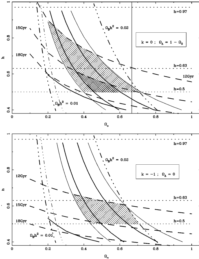
Figure 4 Summary of all the constraints on \Omega_{DM} and h from different observations. (Top) \Omega_\Lambda + \Omega_0 = 1 ; (bottom) \Omega_\Lambda = 0, \Omega_0 < 1 , with \Omega_0 = \Omega_B + \Omega_{DM} . (Thick, broken lines) Models of constant age, with t_0 = (12 \text{ Gyr}, 18 \text{ Gyr}) ; (thick, unbroken lines) the region allowed by cluster abundance; (thin lines) the extent to which this region can be enlarged due to the uncertainty in COBE measurements of the temperature anisotropy. (Thick dash-triple dot lines) The constraints from primordial deuterium abundance (for \Omega_b h^2 = 0.02 and 0.01 ); (thin line) from deuterium abundance at high redshift; (thick, unbroken line) from the abundance of high redshift objects, obtained by requiring that a mass scale 10^{11} M_\odot should go nonlinear at z \geq 2 . (Cross-hatched area) The region allowed without taking uncertainty in COBE normalization into account. If the uncertainties in the observations are pushed to the extreme limits, then the allowed parameter space corresponds to the shaded region. A somewhat less conservative interpretation of observations will lead to a much smaller allowed region (cross-hatched area). Here we have not used the bounds arising from values of the deceleration parameter and observation of deuterium abundance at high redshift. (For details, see Bagla et al. 1996.)
