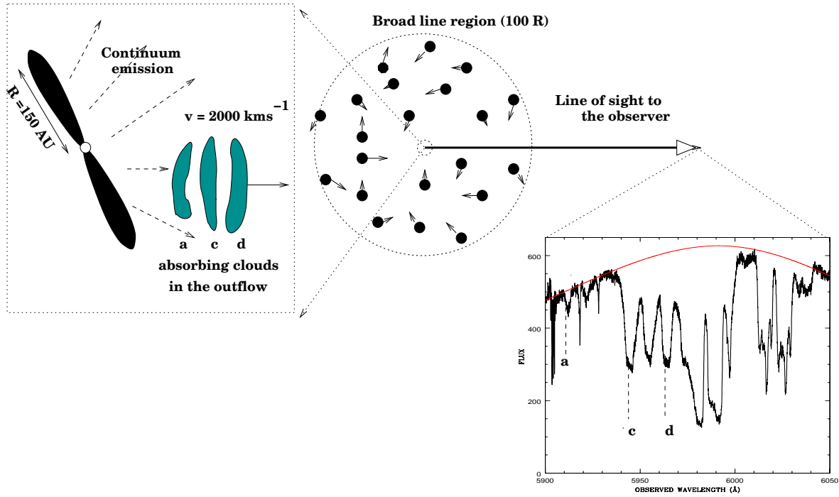
Figure 5. Qualitative sketch of the relative position of the absorbing gas compared to the flux emitting region. The fact that some of the components of the outflow from Q 1511+091 cover only part of the source of continuum suggests that the absorbing gas is close to the continuum emission region. Typically the continuum is believed to originate from a region of size R \sim 150 AU. Reverberation mapping studies of AGNs indicate that the broad emission lines are produced by a region of radius at least 100 times that of the continuum emitting region. Thus it is most likely that at least part of the observed flow originate close to the inner boundary of the broad emission line region.
