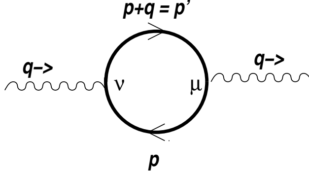
Figure 2. One-loop diagram for the vacuum polarization.
